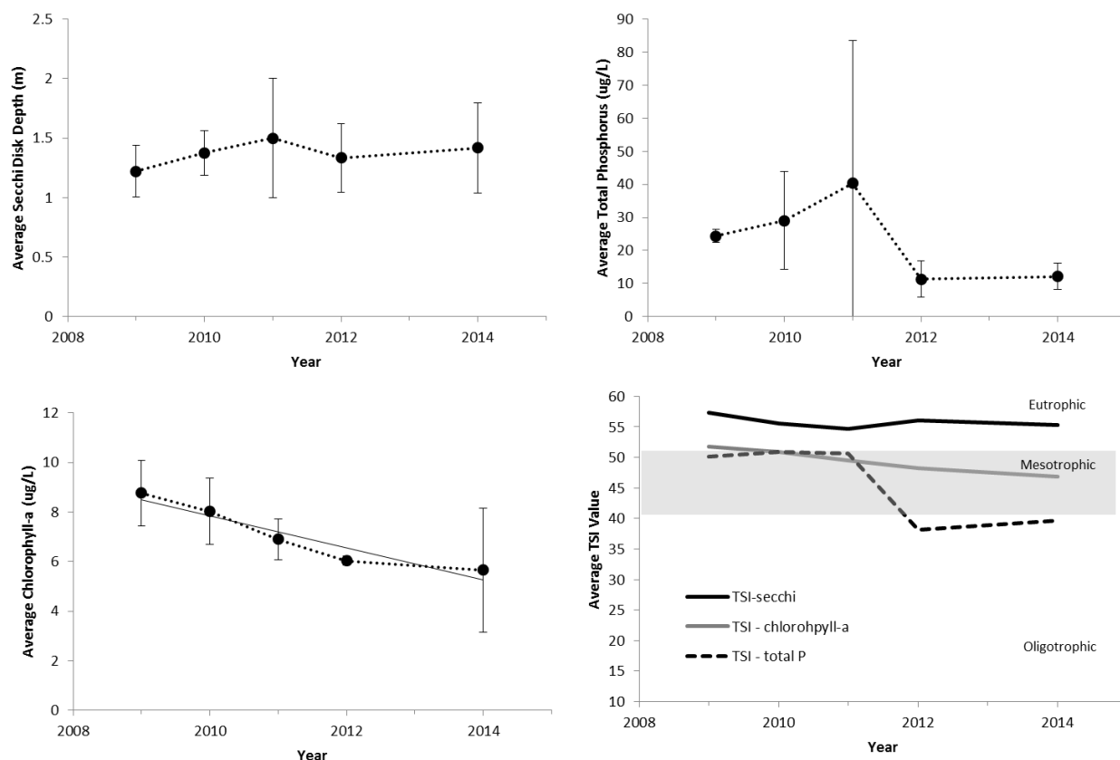
Figure 3. The annual average values of epilimnetic trophic indicators of Jordan Lake, 2009-2014. (A) Secchi disk transparency, (B) total phosphorus concentration, (C) chlorophyll-a concentration, and (D) Carlson's Trophic Status Index. Vertical bars represent one standard deviation of the mean. Significant trends ( P \leq 0.05 ) are noted with a trend line.
