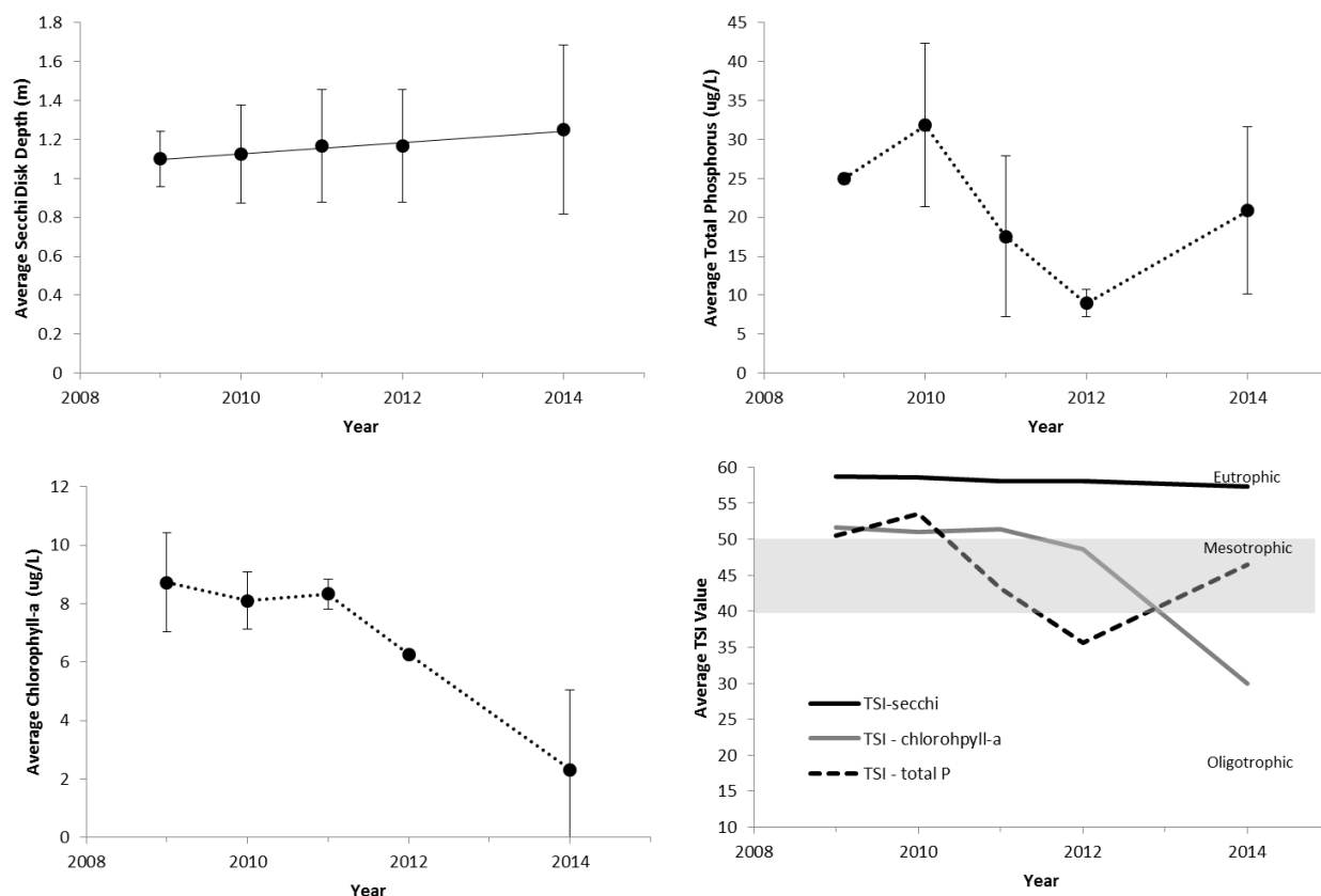
Figure 3. The annual average values of epilimnetic trophic indicators of Amber Lake, 2009-2014. (A) Secchi disk transparency, (B) total phosphorus concentration, (C) chlorophyll-a concentration, and (D) Carlson's Trophic Status Index. Vertical bars represent one standard deviation of the mean. Significant trends ( P \leq 0.05 ) are noted with a trend line.
