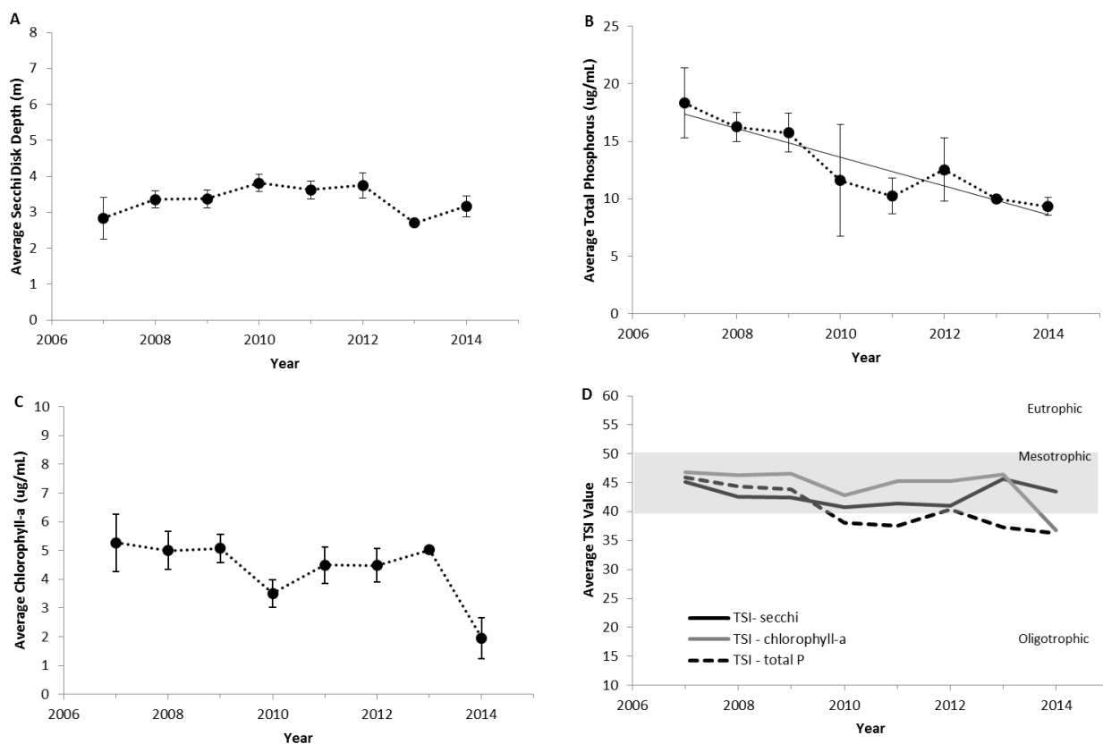
Figure 3. The annual average values of epilimnetic trophic indicators of Upper Chateaugay Lake, 2007-2014. (A) Secchi disk transparency, (B) total phosphorus concentration, (C) chlorophyll-a concentration, and (D) Carlson's Trophic Status Index. Vertical bars represent one standard deviation of the mean. Significant trends ( P \leq 0.05 ) are noted with a trend line.
