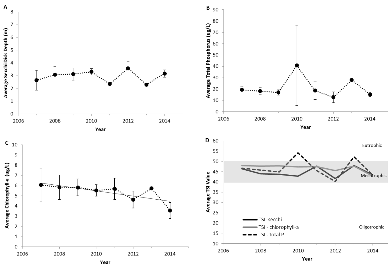
Figure 3. The annual average values of epilimnetic trophic indicators of Lower Chateaugay Lake, 2007-2014. (A) Secchi disk transparency, (B) total phosphorus concentration, (C) chlorophyll-a concentration, and (D) Carlson's Trophic Status Index. Vertical bars represent one standard deviation of the mean. Significant trends ( P \leq 0.05 ) are noted with a trend line.
