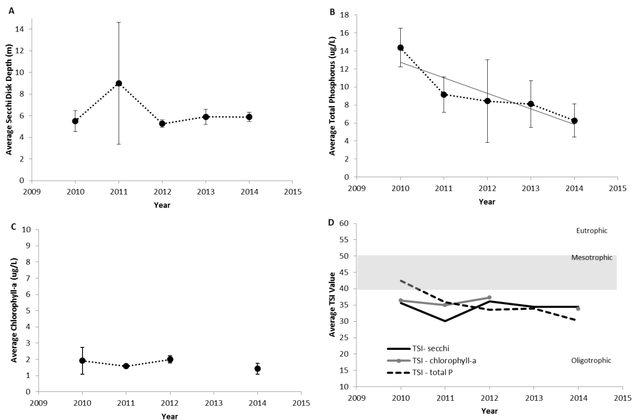
Figure 3. The annual average values of epilimnetic trophic indicators of Thirteenth Lake, 2010-2014. (A) Secchi disk transparency, (B) total phosphorus concentration, (C) chlorophyll-a concentration, and (D) Carlson's Trophic Status Index. Vertical bars represent one standard deviation of the mean. Significant trends ( P \leq 0.05 ) are noted with a trend line.
