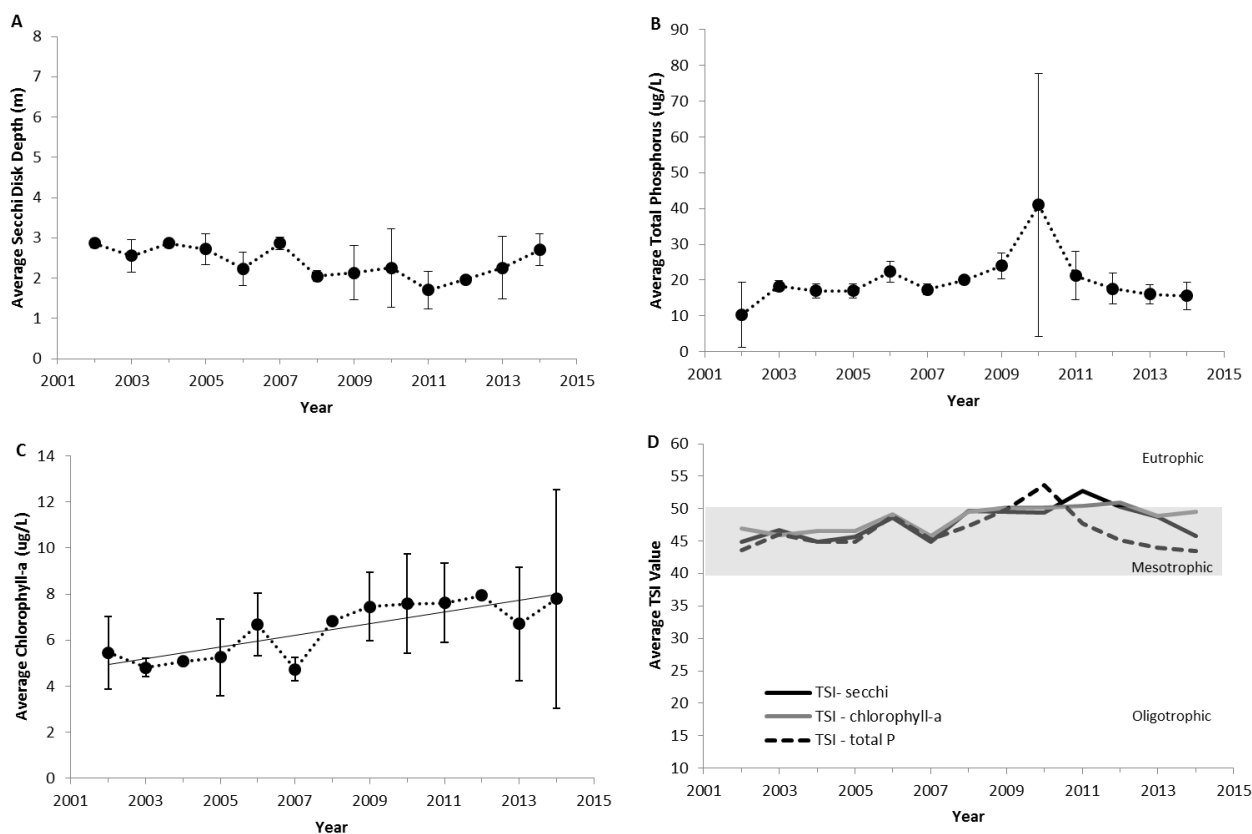
Figure 3. The annual average values of epilimnetic trophic indicators of Snowshoe Pond, 2002-2014. (A) Secchi disk transparency, (B) total phosphorus concentration, (C) chlorophyll-a concentration, and (D) Carlson's Trophic Status Index. Vertical bars represent one standard deviation of the mean. Significant trends ( P \leq 0.05 ) are noted with a trend line.
