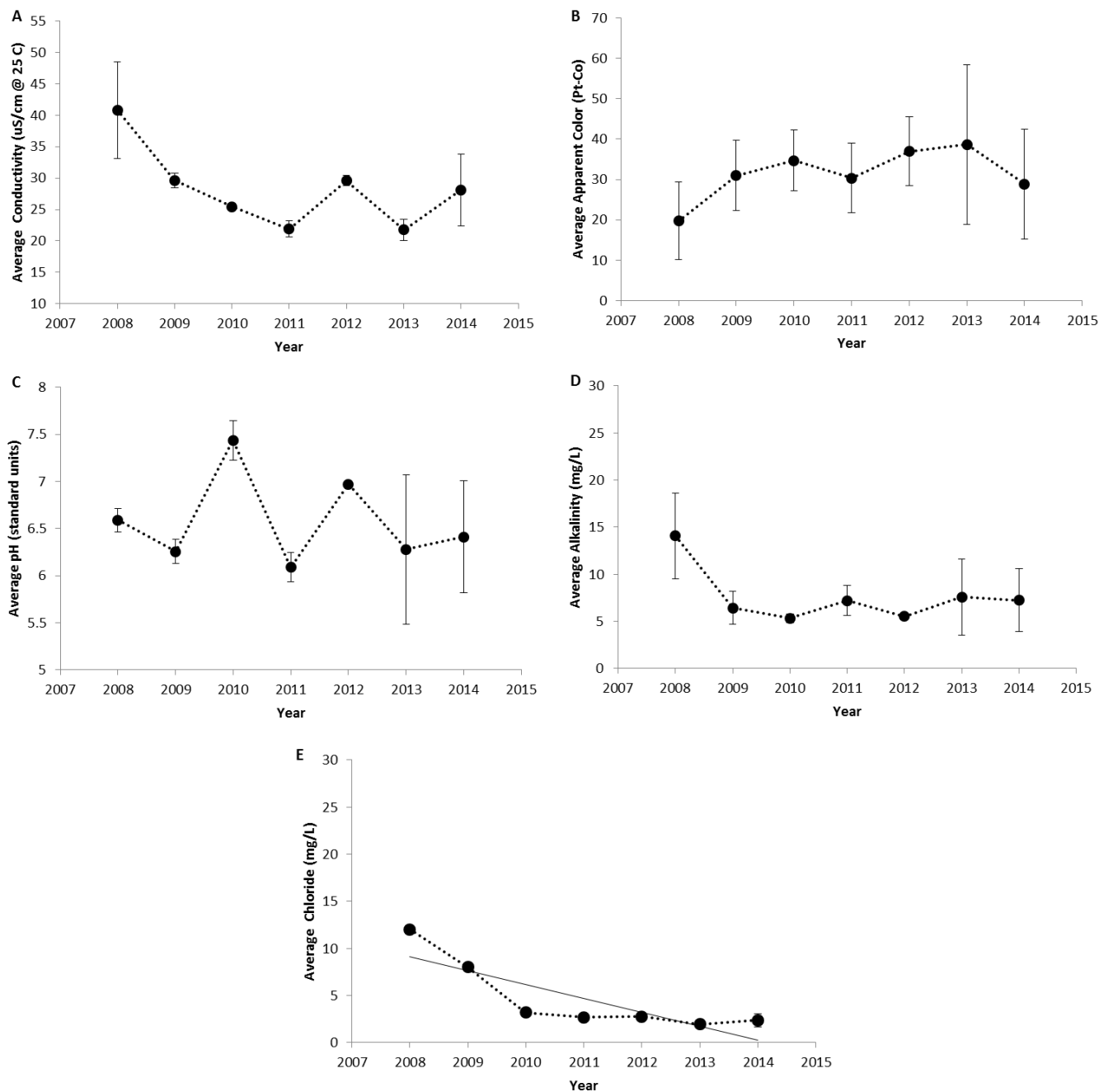
Figure 4. The annual average values of water quality indicators of Simon Pond, 2008-2014. (A) Specific lab conductivity @ 25 C, (B) apparent color, (C) pH, (D) total alkalinity, and (E) chloride. Vertical bars represent one standard deviation of the mean. Significant trends ( P \leq 0.05 ) are noted with a trend line.
