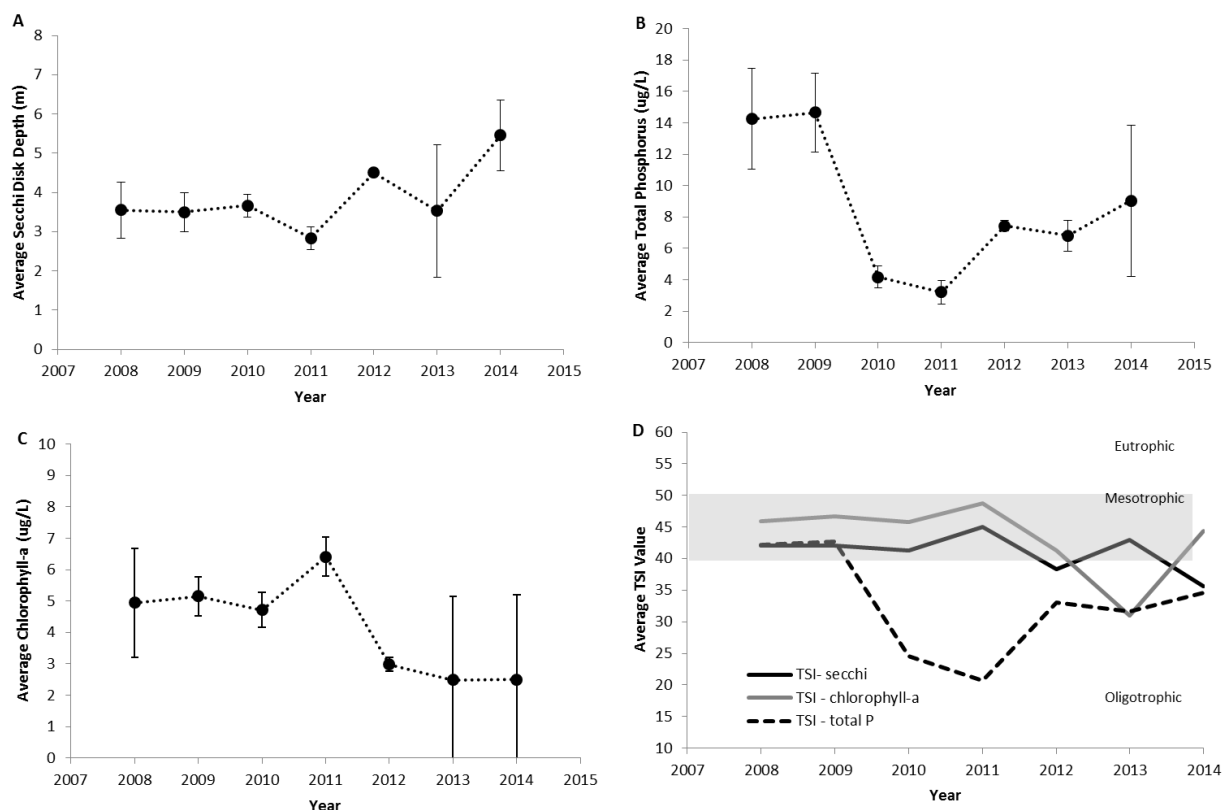
Figure 3. The annual average values of epilimnetic trophic indicators of Simon Pond, 2008-2014. (A) Secchi disk transparency, (B) total phosphorus concentration, (C) chlorophyll-a concentration, and (D) Carlson's Trophic Status Index. Vertical bars represent one standard deviation of the mean. Significant trends ( P \leq 0.05 ) are noted with a trend line.
