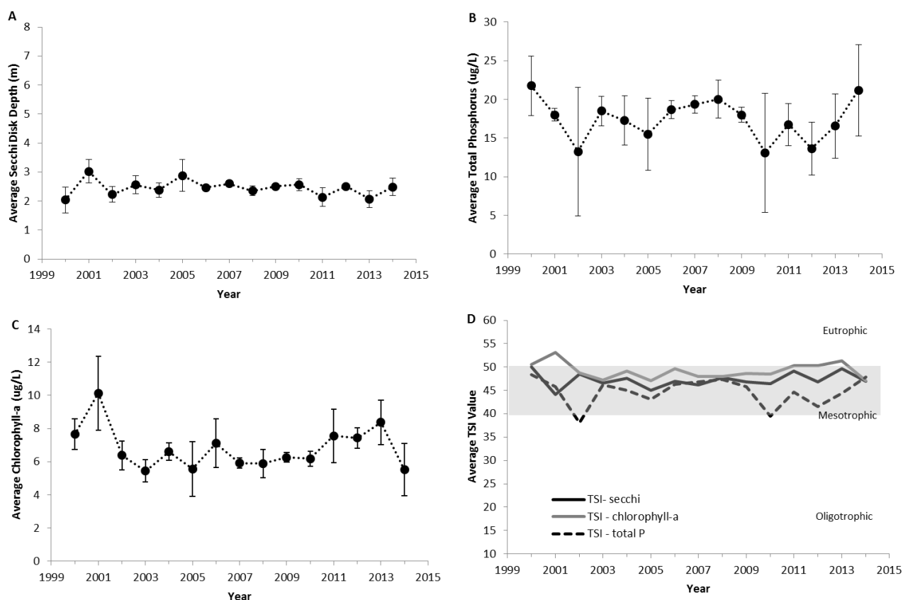
Figure 3. The annual average values of epilimnetic trophic indicators of Osgood Pond, 2000-2014. (A) Secchi disk transparency, (B) total phosphorus concentration, (C) chlorophyll-a concentration, and (D) Carlson's Trophic Status Index. Vertical bars represent one standard deviation of the mean. Significant trends ( P \leq 0.05 ) are noted with a trend line.
