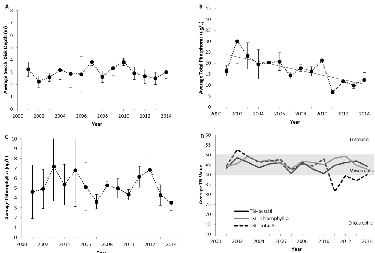
Figure 3. The annual average values of epilimnetic trophic indicators of Lake of the Pines, 2001-2014. (A) Secchi disk transparency, (B) total phosphorus concentration, (C) chlorophyll-a concentration, and (D) Carlson's Trophic Status Index. Vertical bars represent one standard deviation of the mean. Significant trends ( P\leq 0.05 ) are noted with a trend line.
