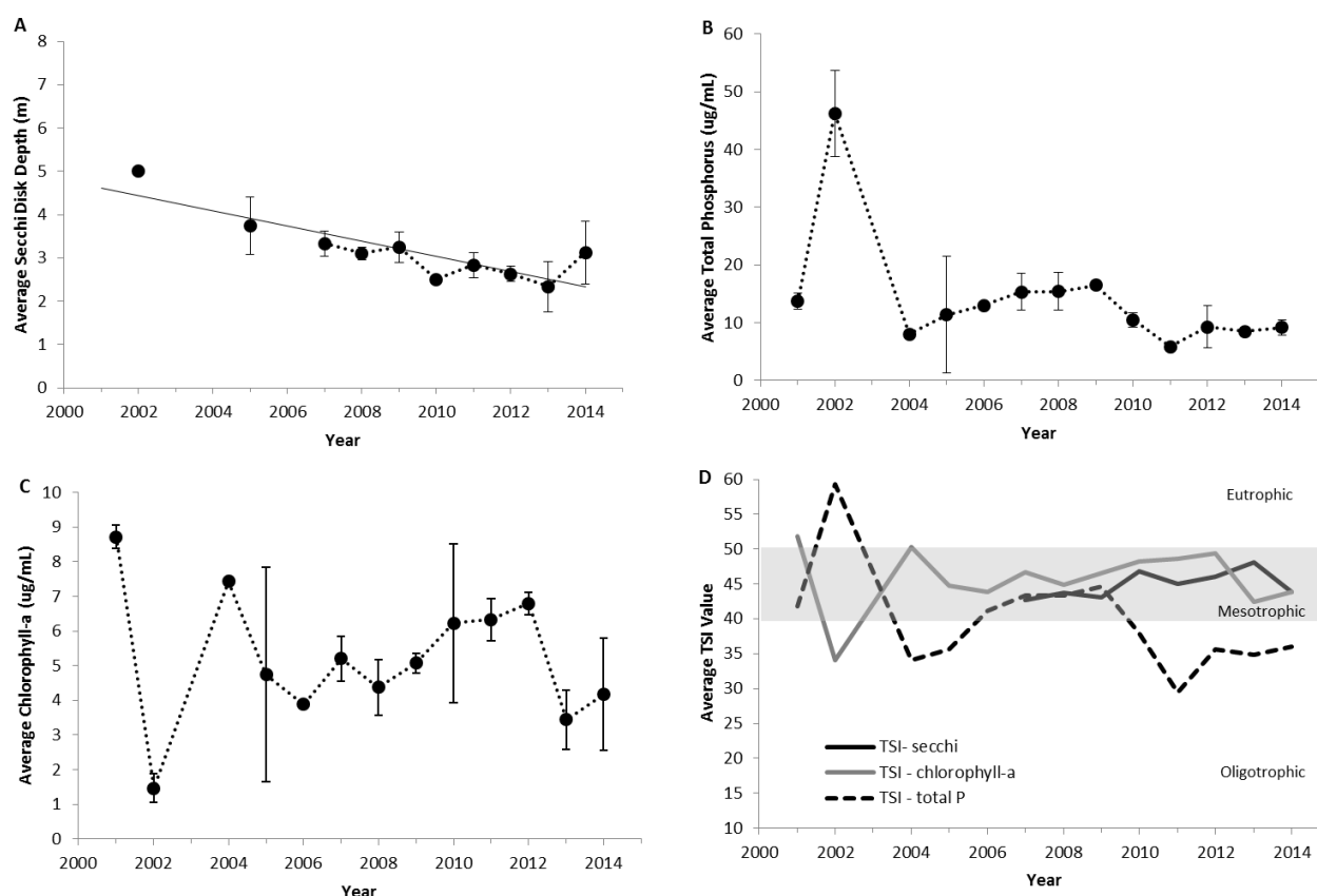
Figure 3. The annual average values of epilimnetic trophic indicators of Lower Saranac Lake, 2001-2014. (A) Secchi disk transparency, (B) total phosphorus concentration, (C) chlorophyll-a concentration, and (D) Carlson's Trophic Status Index. Vertical bars represent one standard deviation of the mean. Significant trends ( P \leq 0.05 ) are noted with a trend line.
