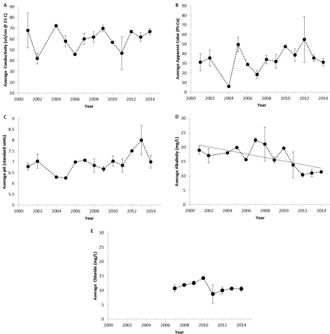
Figure 4. The annual average values of water quality indicators of Lower Saranac Lake, 2001-2014. (A) Specific lab conductivity @ 25 C, (B) apparent color, (C) pH, (D) total alkalinity, and (E) chloride. Vertical bars represent one standard deviation of the mean. Significant trends ( P \leq 0.05 ) are noted with a trend line.
