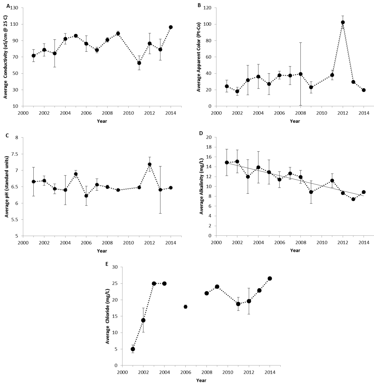
Figure 4. The annual average values of water quality indicators of Balfour Lake, 2001-2014. (A) Specific lab conductivity @ 25 C, (B) apparent color, (C) pH, (D) total alkalinity, and (E) chloride. Vertical bars represent one standard deviation of the mean. Significant trends ( P \leq 0.05 ) are noted with a trend line.
