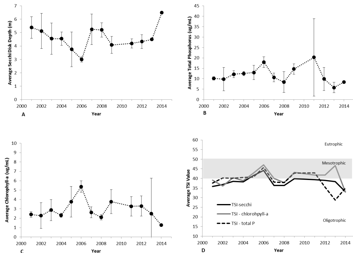
Figure 3. The annual average values of epilimnetic trophic indicators of Balfour Lake, 2001-2014. (A) Secchi disk transparency, (B) total phosphorus concentration, (C) chlorophyll-a concentration, and (D) Carlson's Trophic Status Index. Vertical bars represent one standard deviation of the mean. Significant trends ( P \leq 0.05 ) are noted with a trend line.
