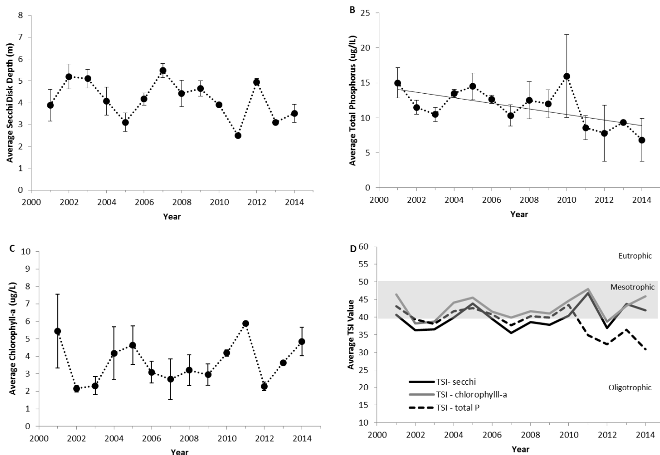
Figure 3. The annual average values of epilimnetic trophic indicators of Catlin Lake, 2001-2014. (A) Secchi disk transparency, (B) total phosphorus concentration, (C) chlorophyll-a concentration, and (D) Carlson's Trophic Status Index. Vertical bars represent one standard deviation of the mean. Significant trends ( P\leq 0.05 ) are noted with a trend line.
