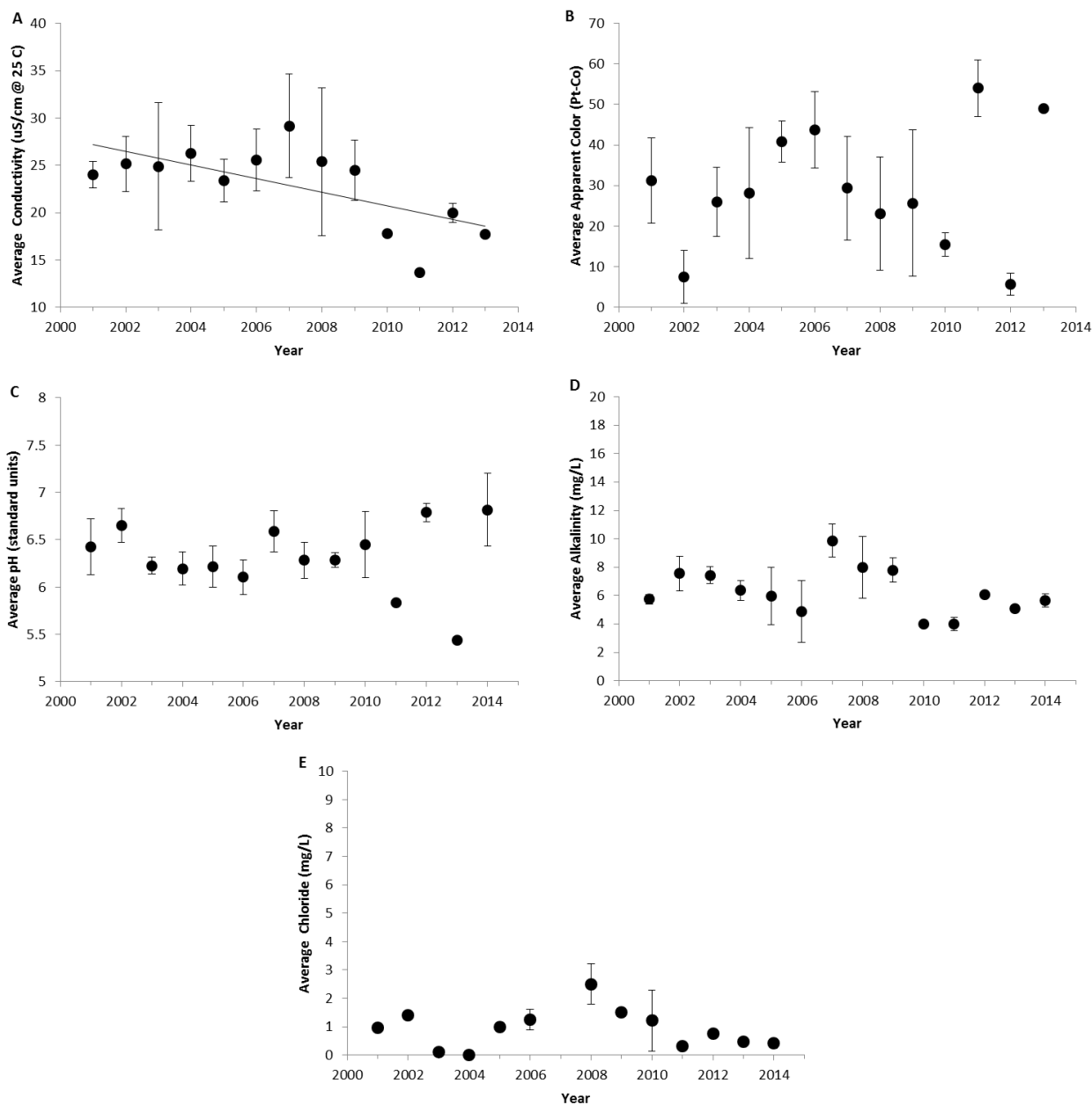
Figure 4. The annual average values of water quality indicators of Arbutus Lake, 2001-2014. (A) Specific lab conductivity @ 25 C, (B) apparent color, (C) pH, (D) total alkalinity, and (E) chloride. Vertical bars represent one standard deviation of the mean. Significant trends ( P \leq 0.05 ) are noted with a trend line.
