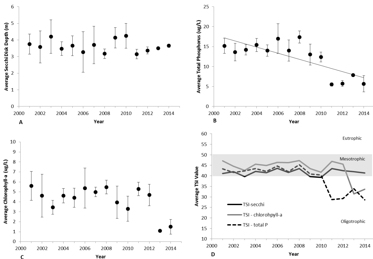
Figure 3. The annual average values of epilimnetic trophic indicators of Arbutus Lake, 2001-2014. (A) Secchi disk transparency, (B) total phosphorus concentration, (C) chlorophyll-a concentration, and (D) Carlson's Trophic Status Index. Vertical bars represent one standard deviation of the mean. Significant trends ( P \leq 0.05 ) are noted with a trend line.
