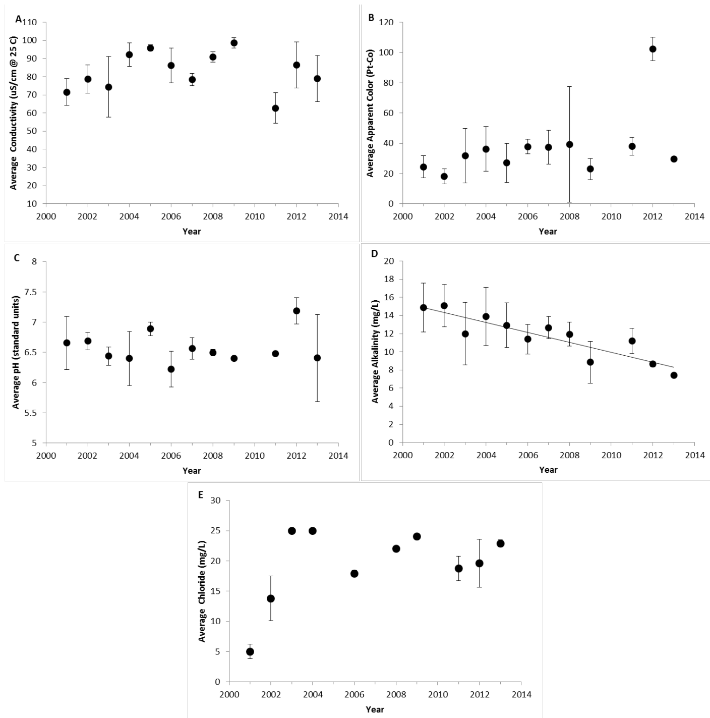
Figure 4. The annual average values of water quality indicators of Balfour Lake, 2001-2013. (A) Specific lab conductivity @ 25°C, (B) apparent color, (C) pH, (D) total alkalinity, and (E) chloride concentration. Vertical bars represent one standard deviation of the mean. Significant trends ( P < 0.05 ) are noted with a trend line.
