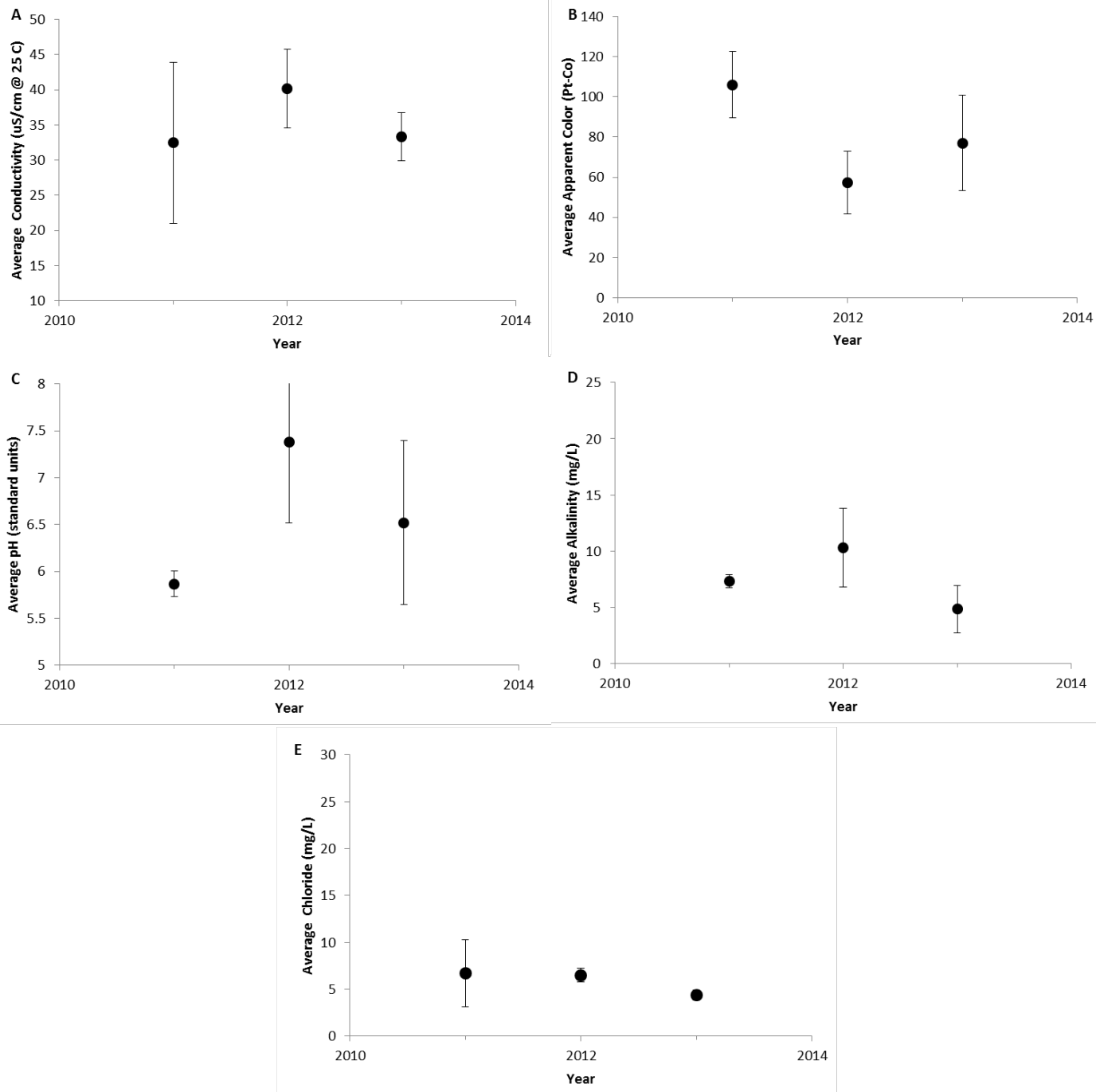
Figure 4. The annual average values of water quality indicators of Lake Durant, 2011-2013. (A) Specific lab conductivity @ 25°C, (B) apparent color, (C) pH, (D) total alkalinity, and (E) chloride concentration. Vertical bars represent one standard deviation of the mean.
