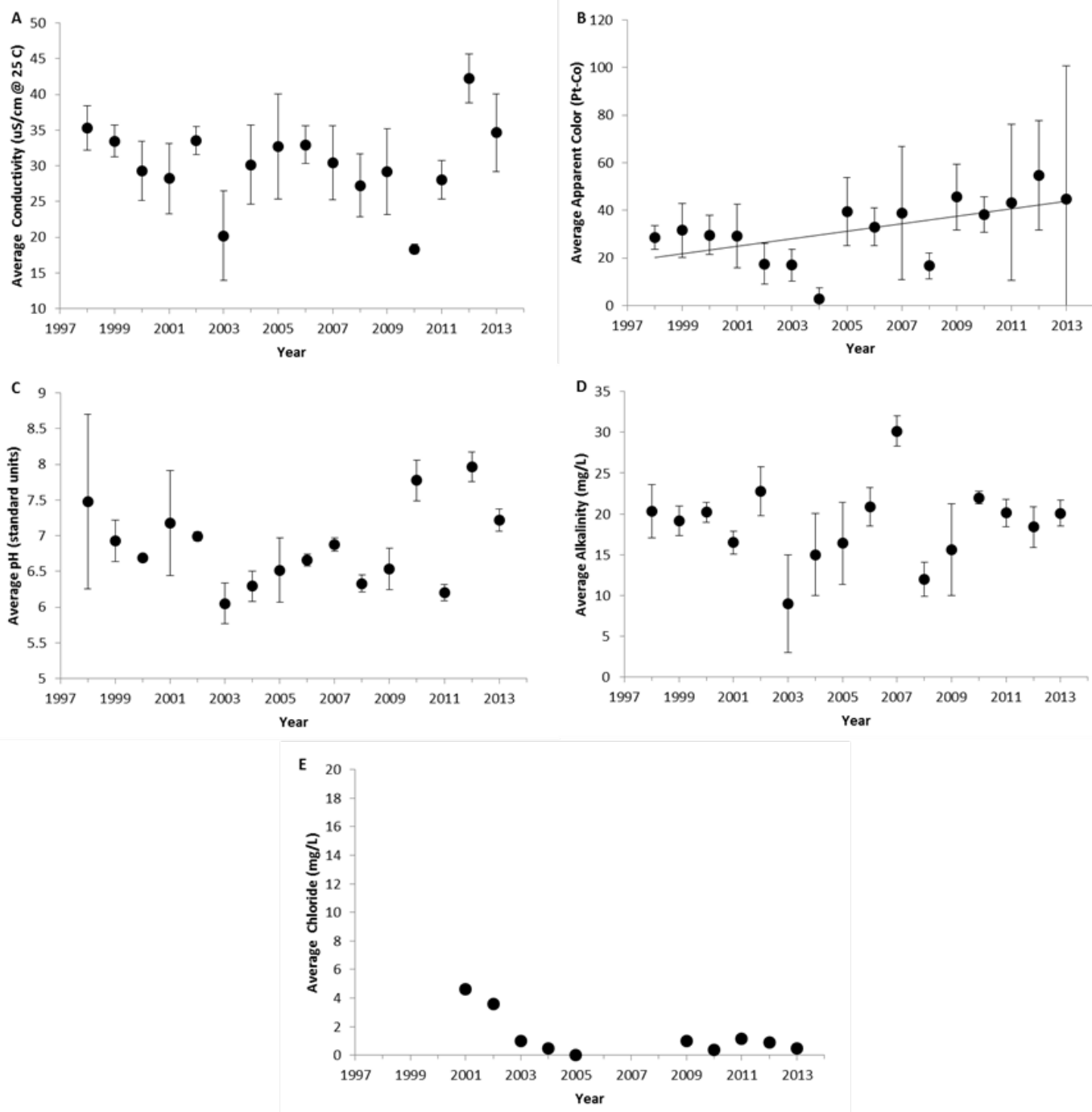
Figure 4. The annual average values of water quality indicators of Oven Mountain Pond, 1998-2013. (A) Specific lab conductivity @ 25°C, (B) apparent color, (C) pH, (D) total alkalinity, and (E) chloride concentration. Vertical bars represent one standard deviation of the mean. Significant trends ( P < 0.05 ) are noted with a trend line.
