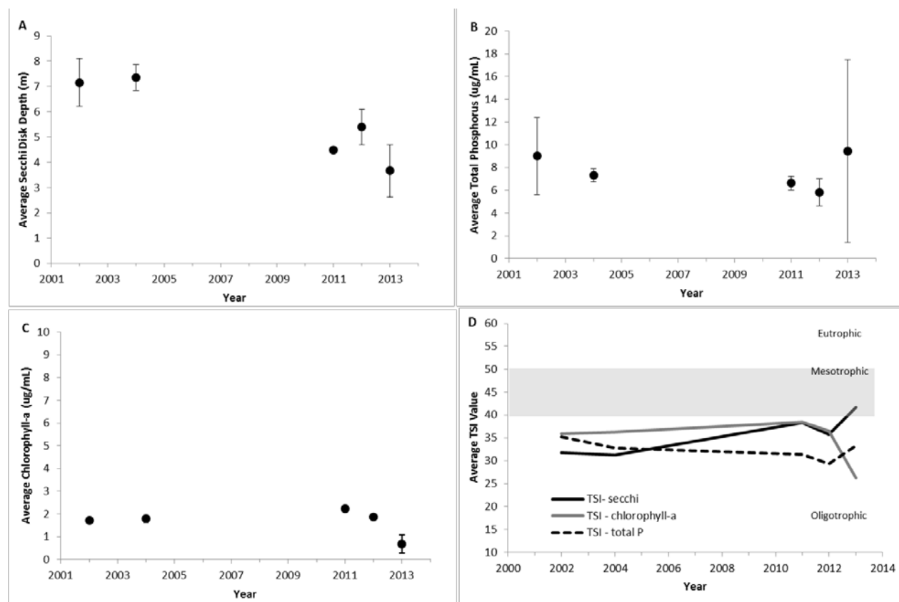
Figure 3. The annual average values of epilimnetic trophic indicators of Upper Cascade Lake, 2002-2013. (A) Secchi disk transparency, (B) total phosphorus concentration, (C) chlorophyll-a concentration, and (D) Carlson's Trophic State Index. Vertical bars represent one standard deviation of the mean. Significant trends ( P < 0.05 ) are noted with a trend line.
