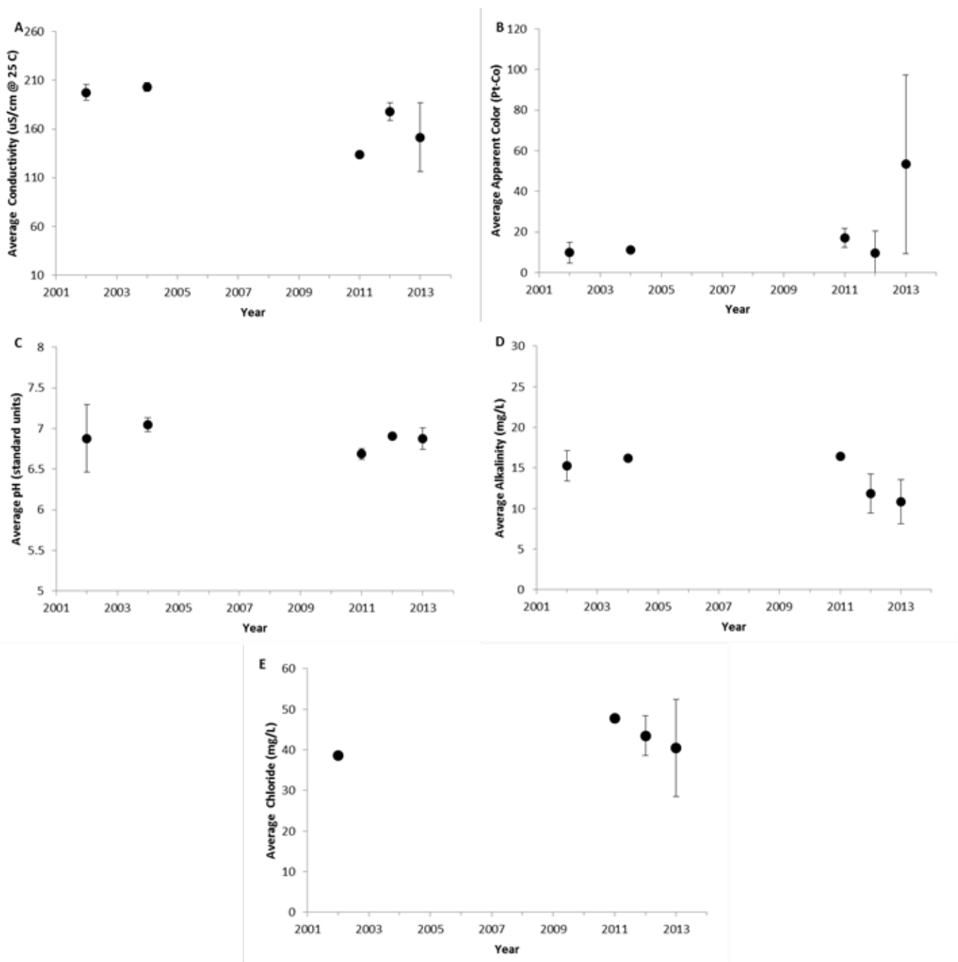
Figure 4. The annual average values of water quality indicators of Upper Cascade Lake, 2002-2013. (A) Specific lab conductivity @ 25°C, (B) apparent color, (C) pH, (D) total alkalinity, and (E) chloride concentration. Vertical bars represent one standard deviation of the mean. Significant trends ( P < 0.05 ) are noted with a trend line.
