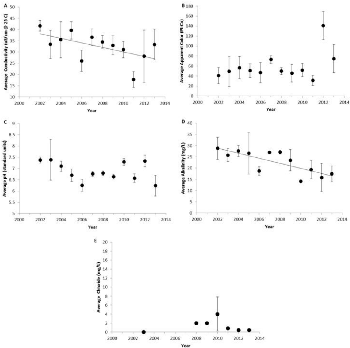
Figure 4. The annual average values of water quality indicators of Snowshoe Pond, 2002-2013. (A) Specific lab conductivity @ 25°C, (B) apparent color, (C) pH, (D) total alkalinity, and (E) chloride concentration. Vertical bars represent one standard deviation of the mean. Significant trends ( P < 0.05 ) are noted with a trend line.
