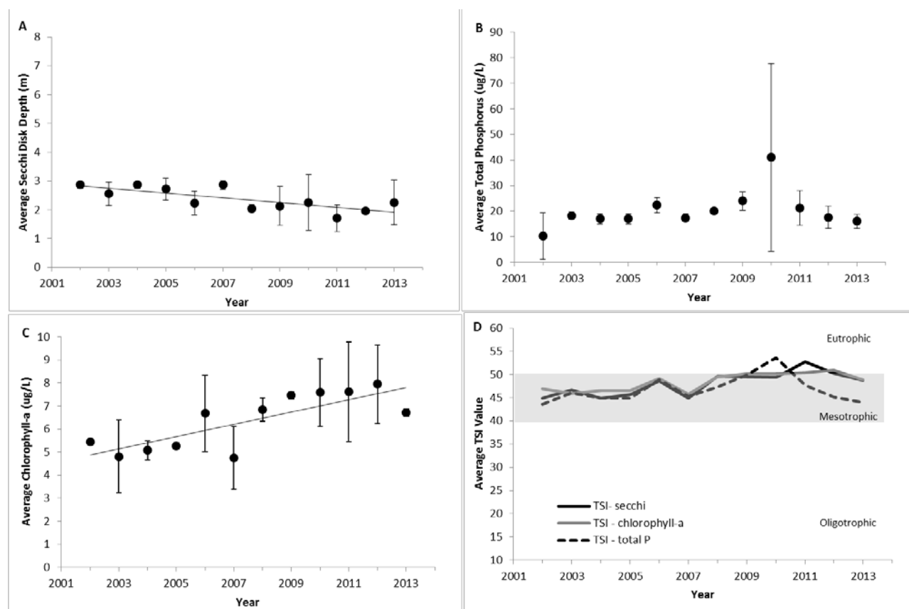
Figure 3. The annual average values of epilimnetic trophic indicators of Snowshoe Pond, 2002-2013. (A) Secchi disk transparency, (B) total phosphorus concentration, (C) chlorophyll-a concentration, and (D) Carlson's Trophic State Index. Vertical bars represent one standard deviation of the mean. Significant trends ( P < 0.05 ) are noted with a trend line.
