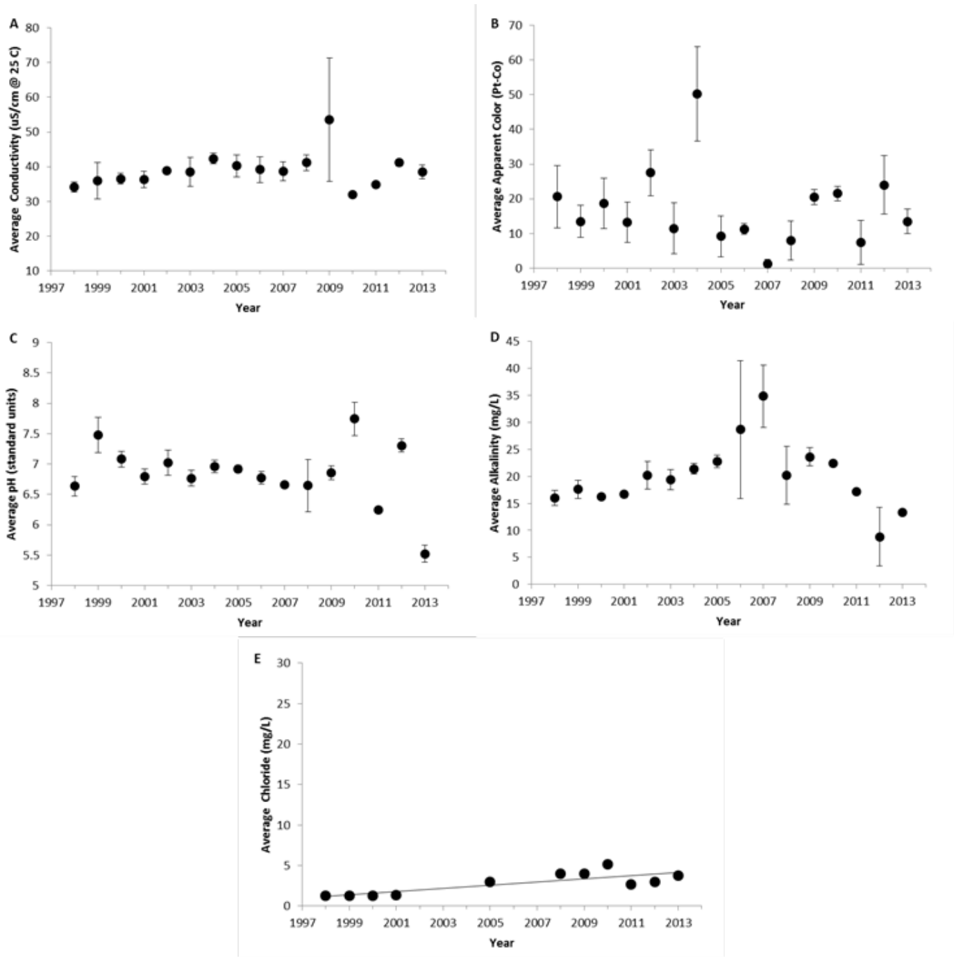
Figure 4. The annual average values of water quality indicators of Silver Lake, 1998-2013. (A) Specific lab conductivity @ 25°C, (B) apparent color, (C) pH, (D) total alkalinity, and (E) chloride concentration. Vertical bars represent one standard deviation of the mean. Significant trends ( P < 0.05 ) are noted with a trend line.
