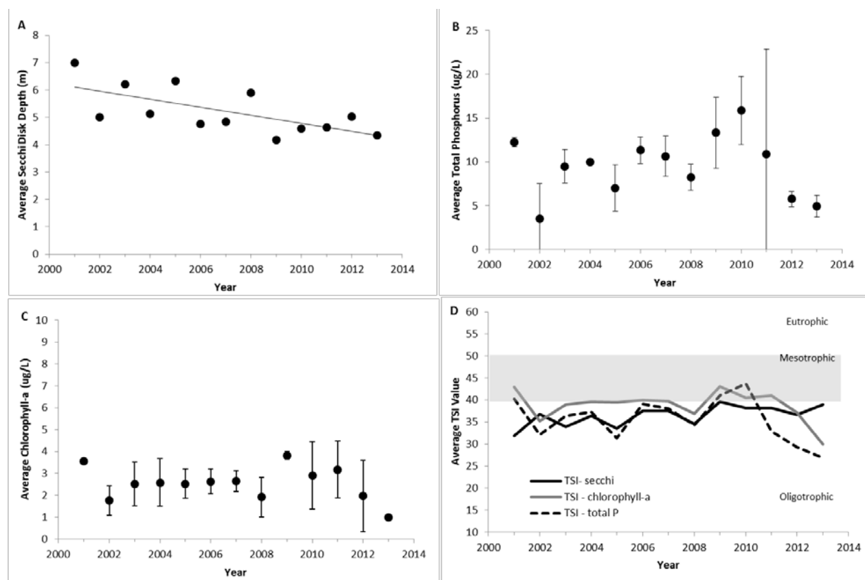
Figure 3. The annual average values of epilimnetic trophic indicators of Pine Lake, 2001-2013. (A) Secchi disk transparency, (B) total phosphorus concentration, (C) chlorophyll-a concentration, and (D) Carlson's Trophic State Index. Vertical bars represent one standard deviation of the mean. Significant trends ( P < 0.05 ) are noted with a trend line.
