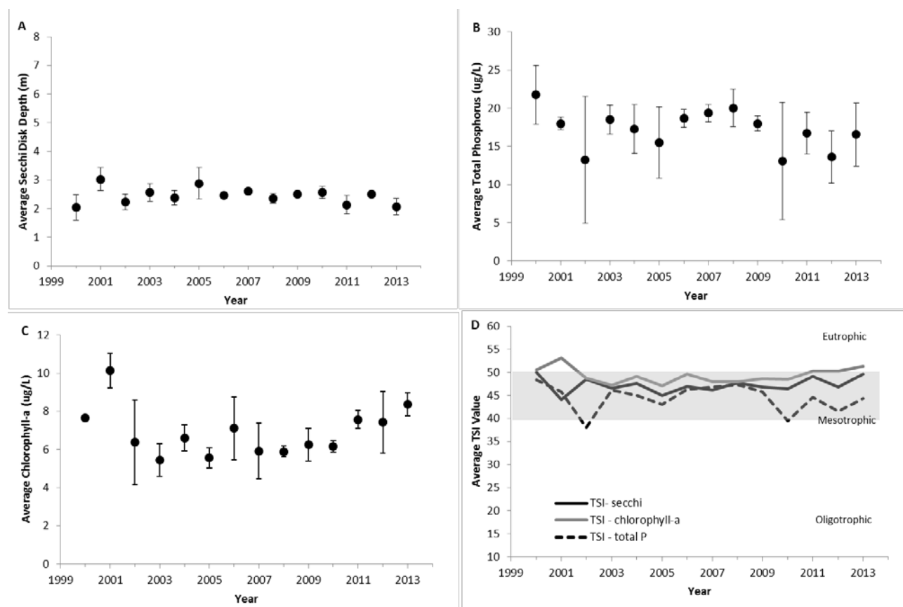
Figure 3. The annual average values of epilimnetic trophic indicators of Osgood Pond, 2000-2013. (A) Secchi disk transparency, (B) total phosphorus concentration, (C) chlorophyll-a concentration, and (D) Carlson's Trophic State Index. Vertical bars represent one standard deviation of the mean. Significant trends ( P < 0.05 ) are noted with a trend line.
