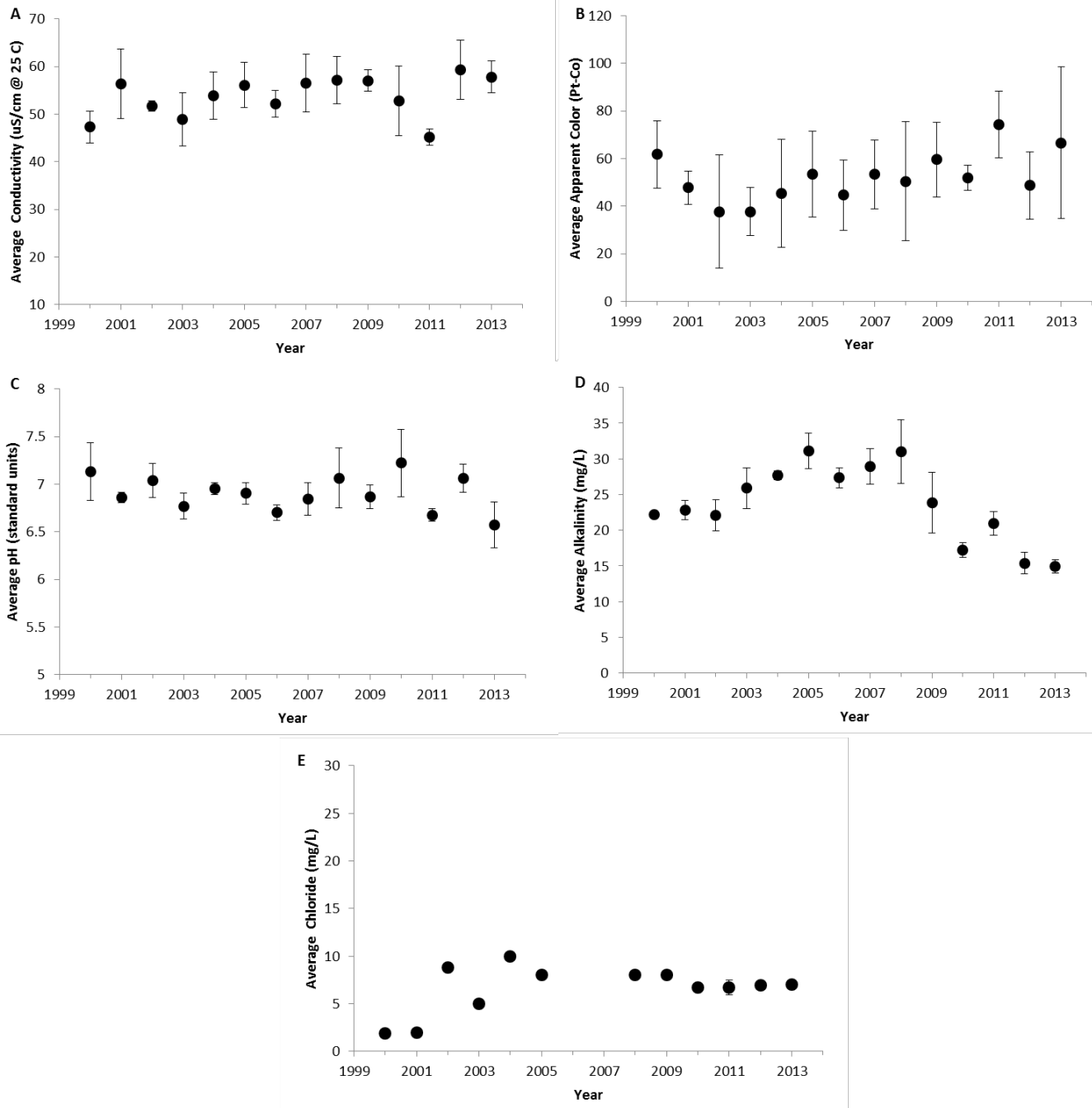
Figure 4. The annual average values of water quality indicators of Osgood Pond, 2000-2013. (A) Specific lab conductivity @ 25°C, (B) apparent color, (C) pH, (D) total alkalinity, and (E) chloride concentration. Vertical bars represent one standard deviation of the mean. Significant trends ( P < 0.05 ) are noted with a trend line.
