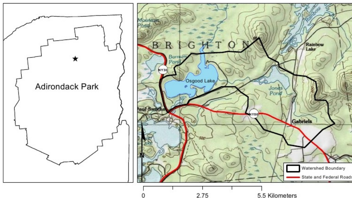
Figure 2. Location and watershed for Osgood Pond.
