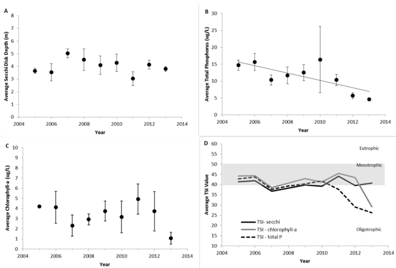
Figure 3. The annual average values of epilimnetic trophic indicators of Moss Lake, 2005-2013. (A) Secchi disk transparency, (B) total phosphorus concentration, (C) chlorophyll-a concentration, and (D) Carlson's Trophic State Index. Vertical bars represent one standard deviation of the mean. Significant trends ( P < 0.05 ) are noted with a trend line.
