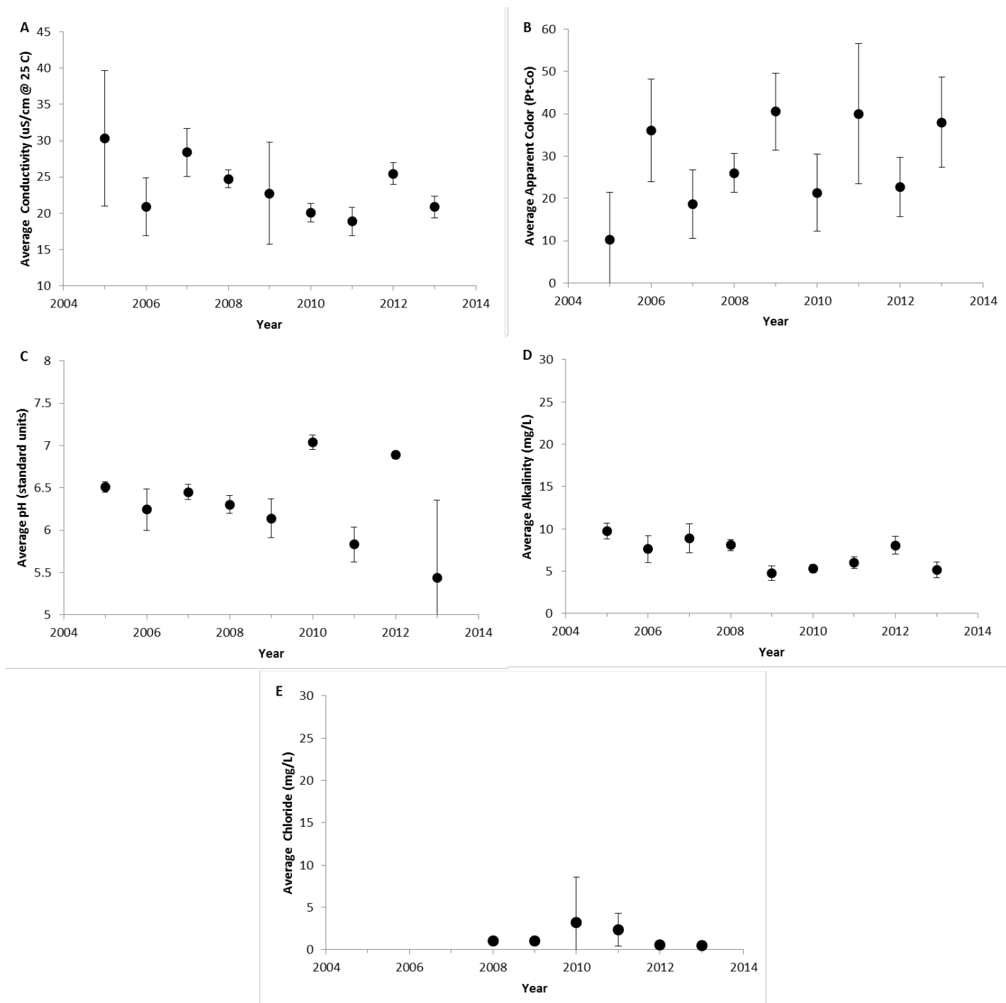
Figure 4. The annual average values of water quality indicators of Moss Lake, 2005-2013. (A) Specific lab conductivity @ 25°C, (B) apparent color, (C) pH, (D) total alkalinity, and (E) chloride concentration. Vertical bars represent one standard deviation of the mean. Significant trends ( P < 0.05 ) are noted with a trend line.
