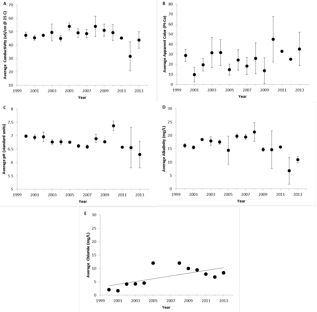
Figure 4. The annual average values of water quality indicators of Middle Saranac Lake, 2000-2013. (A) Specific lab conductivity @ 25°C, (B) apparent color, (C) pH, (D) total alkalinity, and (E) chloride concentration. Vertical bars represent one standard deviation of the mean. Significant trends ( P < 0.05 ) are noted with a trend line.
