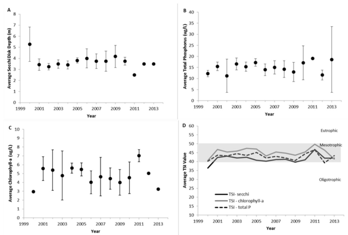
Figure 3. The annual average values of epilimnetic trophic indicators of Middle Saranac Lake, 2000-2013. (A) Secchi disk transparency, (B) total phosphorus concentration, (C) chlorophyll-a concentration, and (D) Carlson's Trophic State Index. Vertical bars represent one standard deviation of the mean. Significant trends ( P < 0.05 ) are noted with a trend line.
