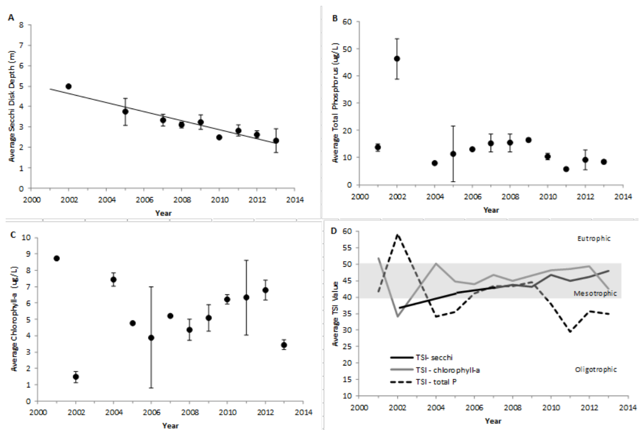
Figure 3. The annual average values of epilimnetic trophic indicators of Lower Saranac Lake, 2001-2013. (A) Secchi disk transparency, (B) total phosphorus concentration, (C) chlorophyll-a concentration, and (D) Carlson's Trophic State Index. Vertical bars represent one standard deviation of the mean. Significant trends ( P < 0.05 ) are noted with a trend line.
