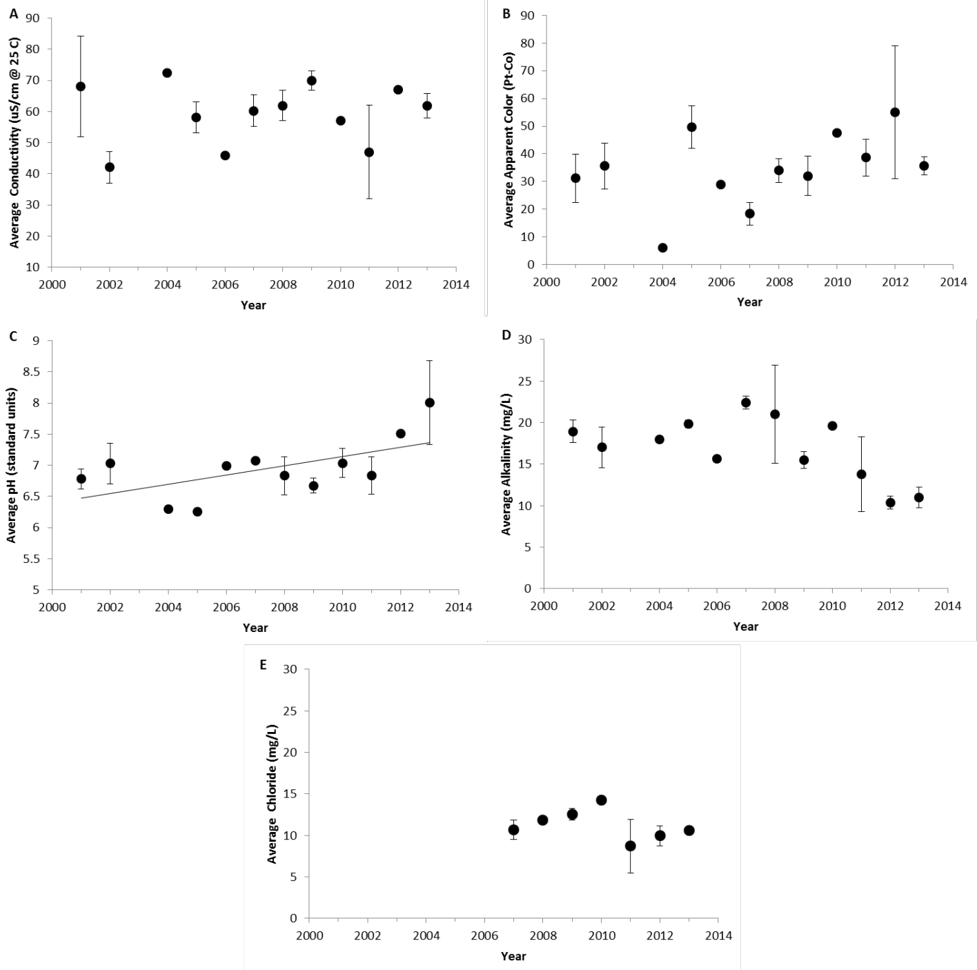
Figure 4. The annual average values of water quality indicators of Lower Saranac Lake, 2001-2013. (A) Specific lab conductivity @ 25°C, (B) apparent color, (C) pH, (D) total alkalinity, and (E) chloride concentration. Vertical bars represent one standard deviation of the mean. Significant trends ( P < 0.05 ) are noted with a trend line.
