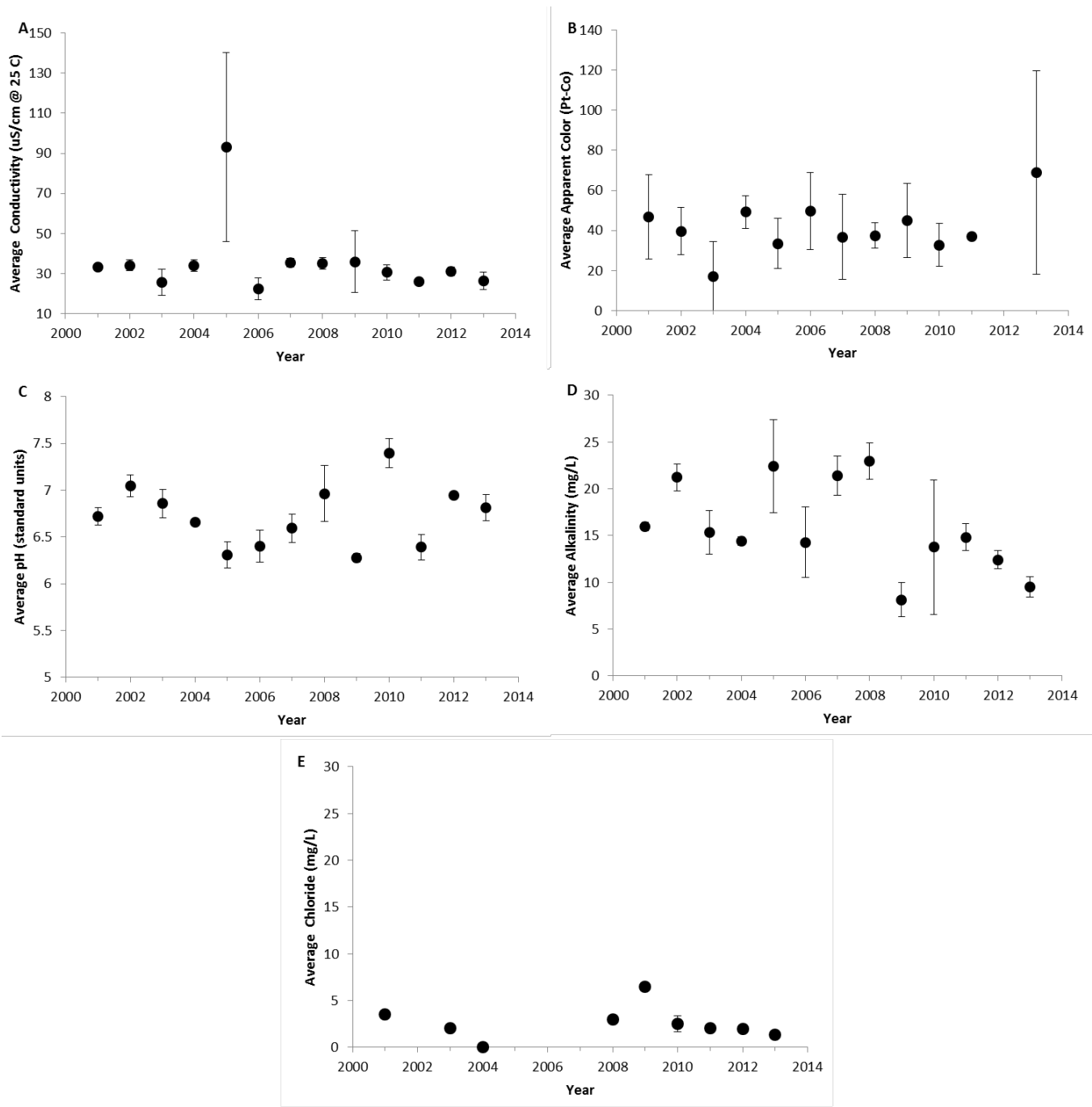
Figure 4. The annual average values of water quality indicators of Lake of the Pines, 2001-2013. (A) Specific lab conductivity @ 25°C, (B) apparent color, (C) pH, (D) total alkalinity, and (E) chloride concentration. Vertical bars represent one standard deviation of the mean. Significant trends ( P < 0.05 ) are noted with a trend line.
