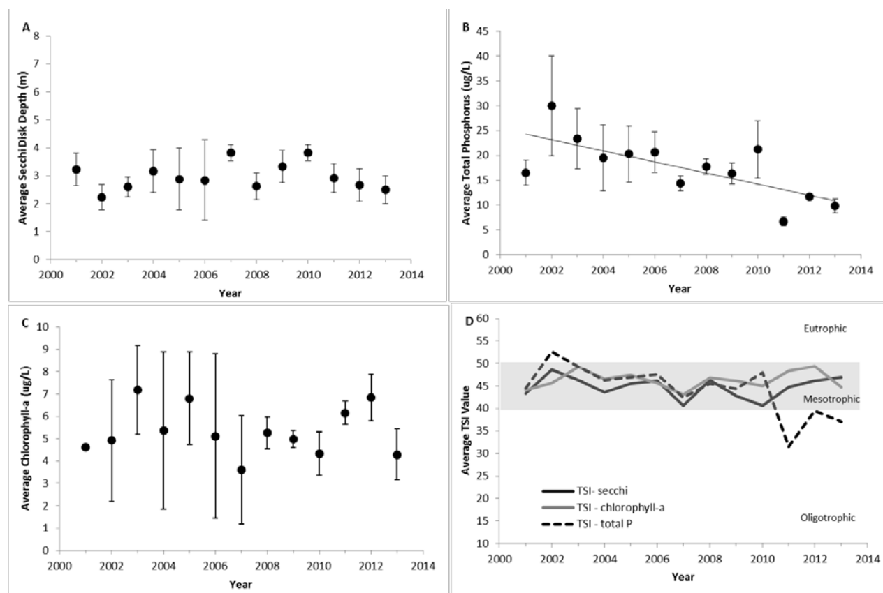
Figure 3. The annual average values of epilimnetic trophic indicators of Lake of the Pines, 2001-2013. (A) Secchi disk transparency, (B) total phosphorus concentration, (C) chlorophyll-a concentration, and (D) Carlson's Trophic State Index. Vertical bars represent one standard deviation of the mean. Significant trends ( P < 0.05 ) are noted with a trend line.
