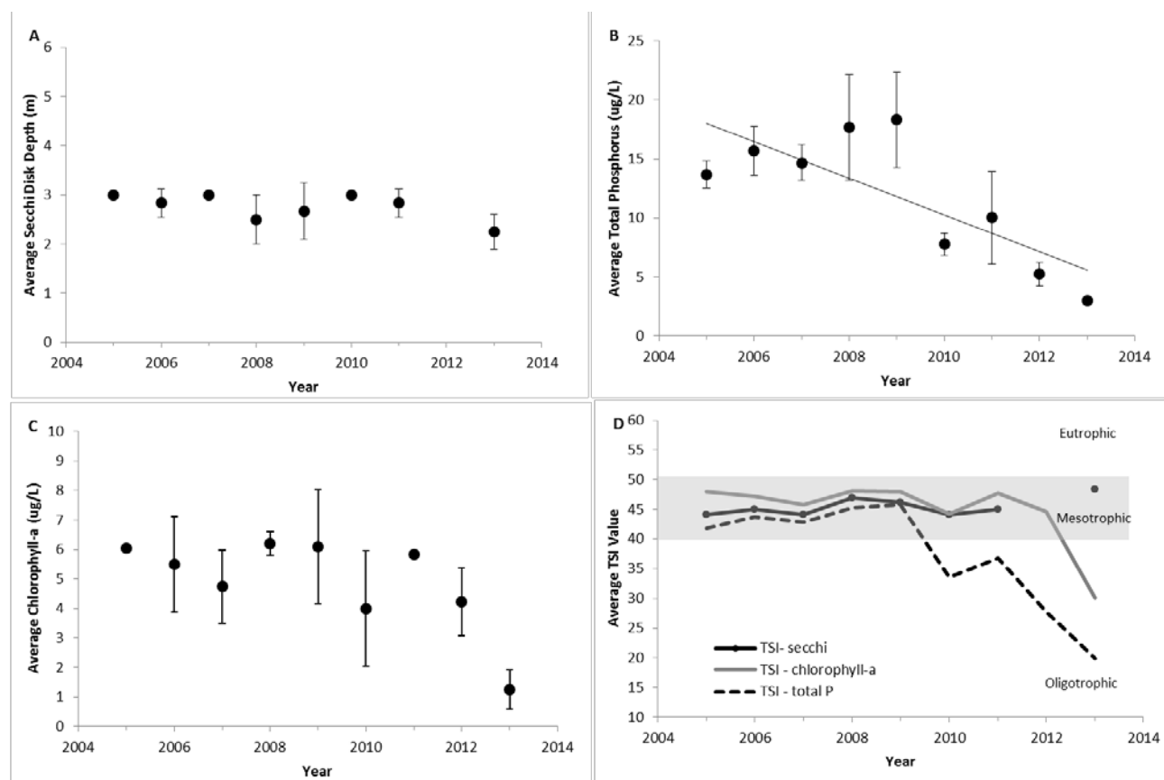
Figure 3. The annual average values of epilimnetic trophic indicators of Lake Abanakee, 2005-2013. (A) Secchi disk transparency, (B) total phosphorus concentration, (C) chlorophyll-a concentration, and (D) Carlson's Trophic State Index. Vertical bars represent one standard deviation of the mean. Significant trends ( P < 0.05 ) are noted with a trend line.
