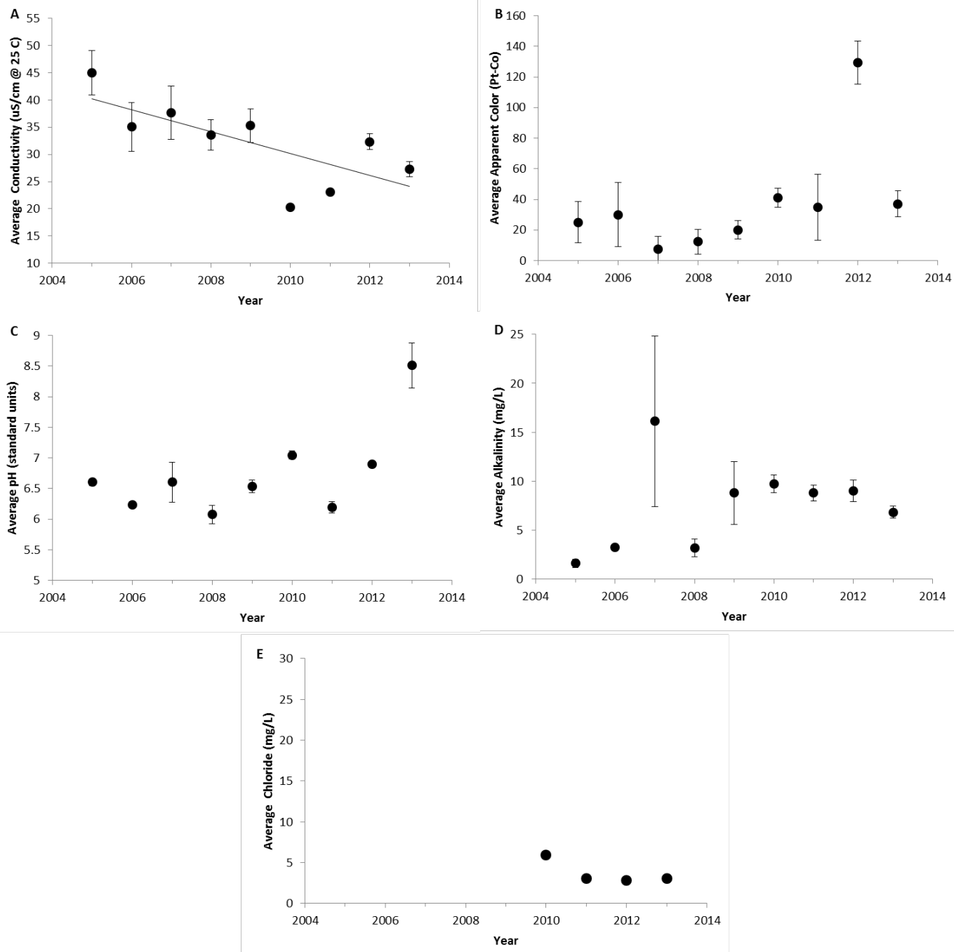
Figure 4. The annual average values of water quality indicators of Lake Abanakee, 2005-2013. (A) Specific lab conductivity @ 25°C, (B) apparent color, (C) pH, (D) total alkalinity, and (E) chloride concentration. Vertical bars represent one standard deviation of the mean. Significant trends ( P < 0.05 ) are noted with a trend line.
