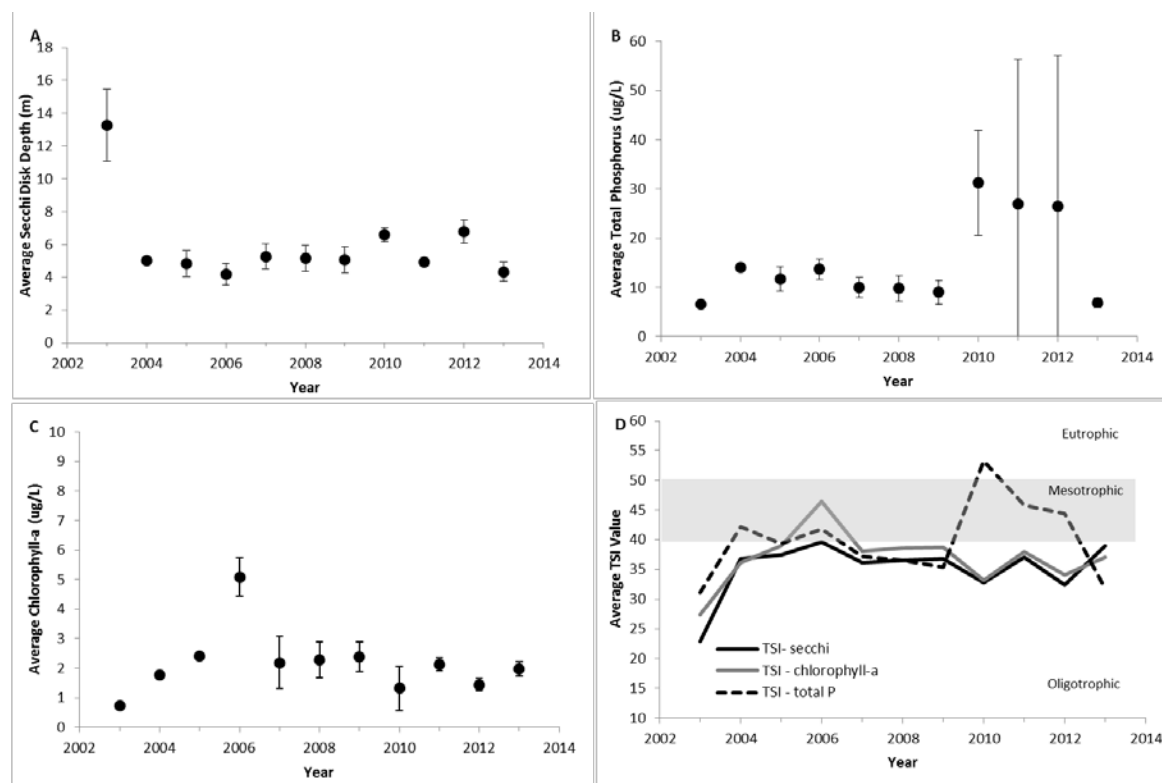
Figure 3. The annual average values of epilimnetic trophic indicators of Kiawassa Lake, 2003-2013. (A) Secchi disk transparency, (B) total phosphorus concentration, (C) chlorophyll-a concentration, and (D) Carlson's Trophic State Index. Vertical bars represent one standard deviation of the mean. Significant trends ( P < 0.05 ) are noted with a trend line.
