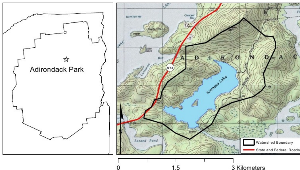
Figure 2. Location and watershed for Kiwassa Lake.
