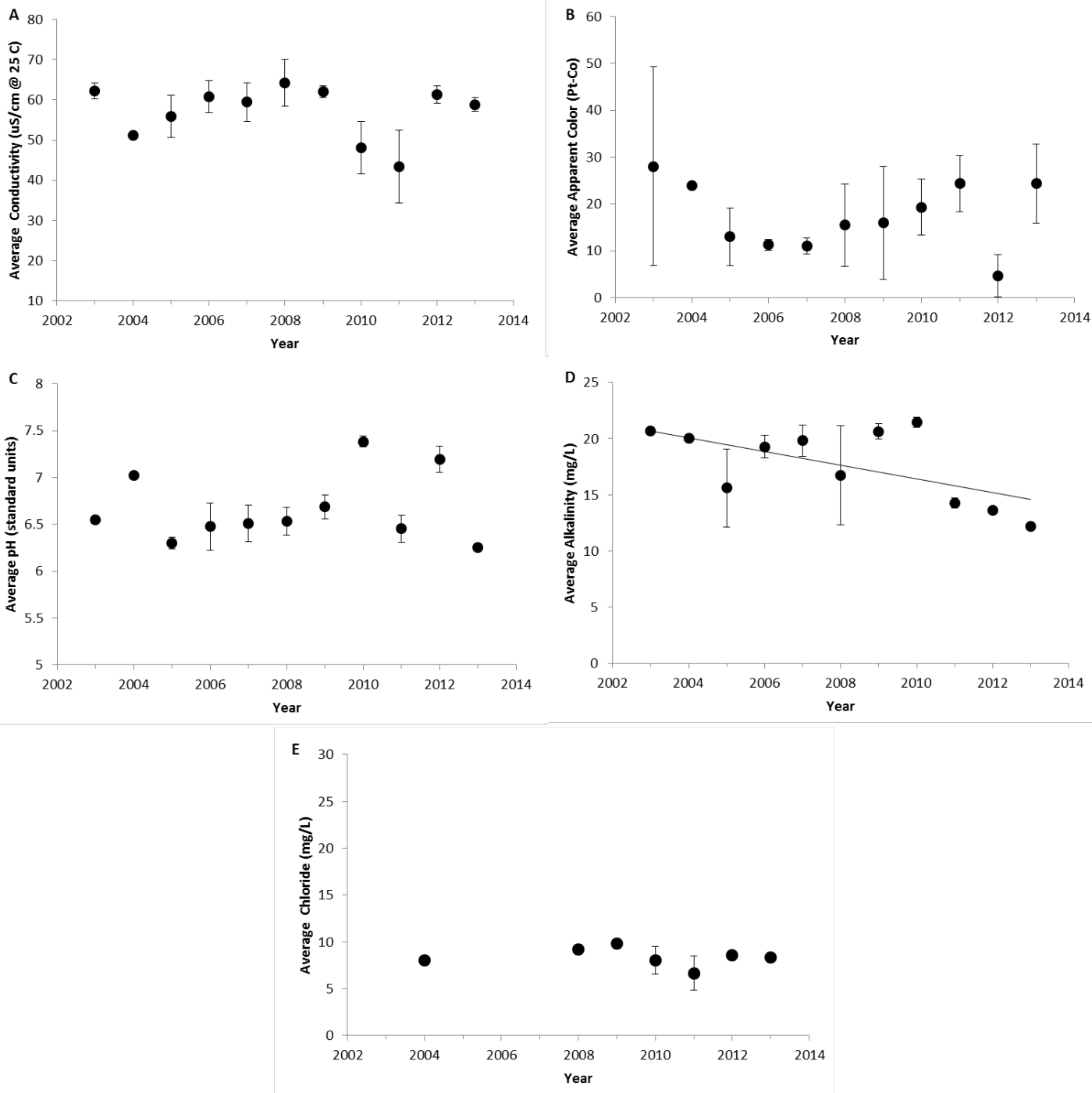
Figure 4. The annual average values of water quality indicators of Kiwassa Lake, 2003-2013. (A) Specific lab conductivity @ 25°C, (B) apparent color, (C) pH, (D) total alkalinity, and (E) chloride concentration. Vertical bars represent one standard deviation of the mean. Significant trends ( P < 0.05 ) are noted with a trend line.
