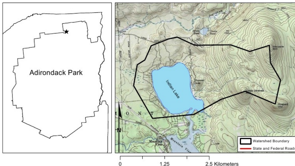
Figure 2. Location and watershed for Indian Lake.
