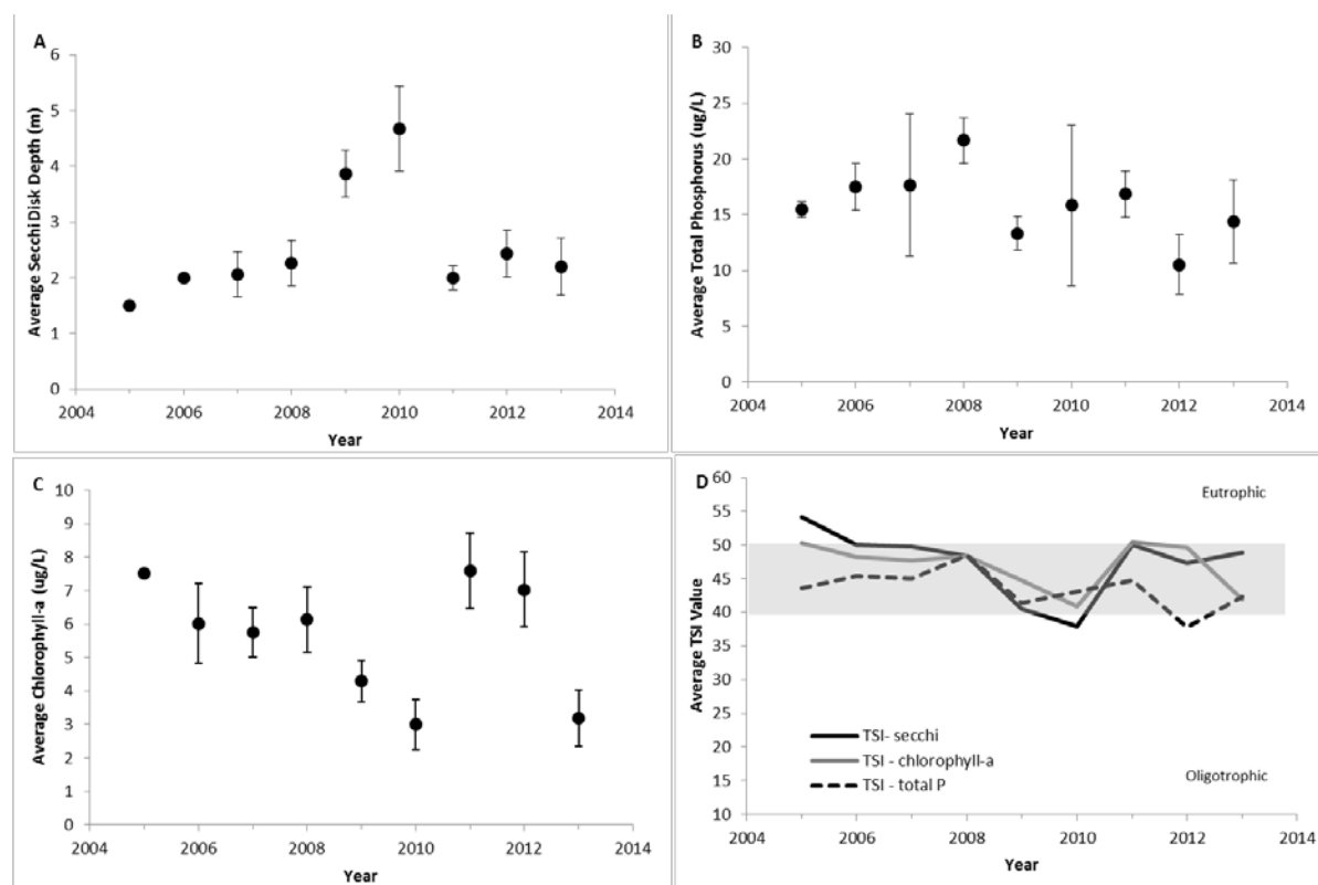
Figure 3. The annual average values of epilimnetic trophic indicators of Indian Lake, 2005-2013. (A) Secchi disk transparency, (B) total phosphorus concentration, (C) chlorophyll-a concentration, and (D) Carlson's Trophic State Index. Vertical bars represent one standard deviation of the mean. Significant trends ( P < 0.05 ) are noted with a trend line.
