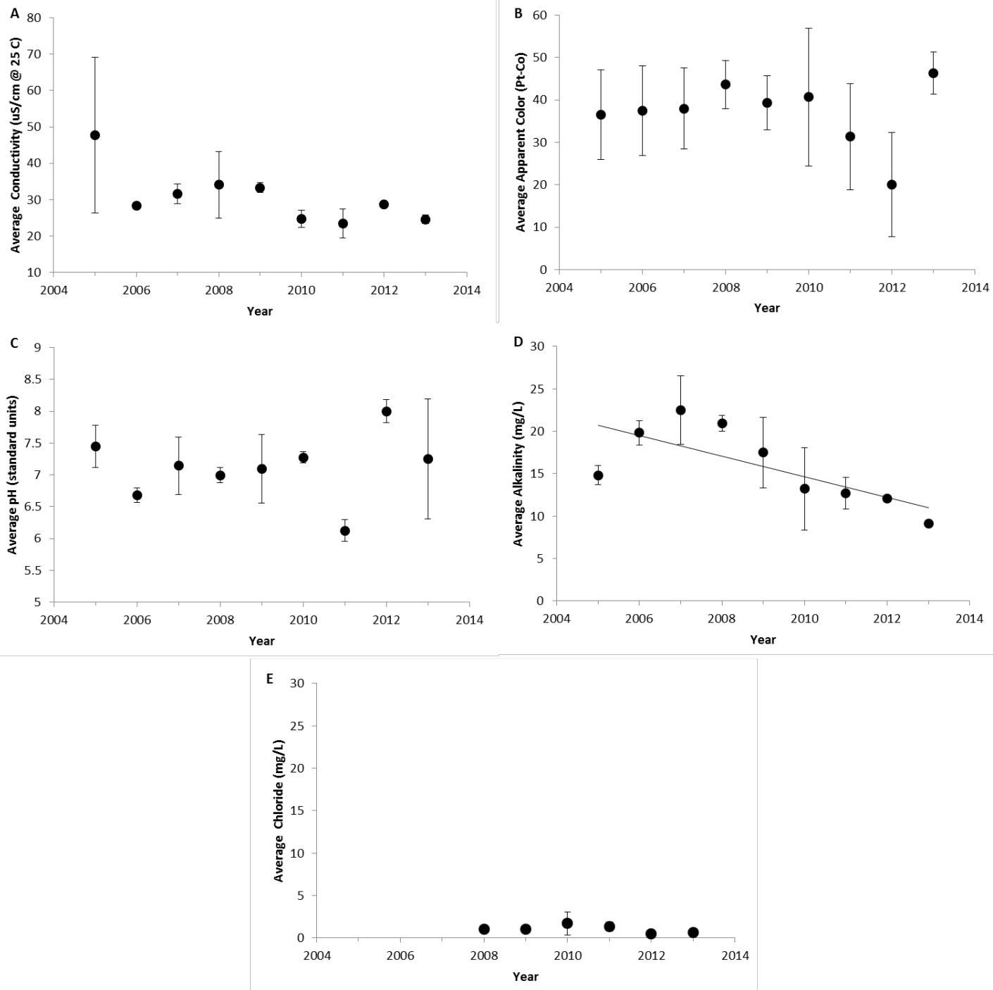
Figure 4. The annual average values of water quality indicators of Indian Lake, 2005-2013. (A) Specific lab conductivity @ 25°C, (B) apparent color, (C) pH, (D) total alkalinity, and (E) chloride concentration. Vertical bars represent one standard deviation of the mean. Significant trends ( P < 0.05 ) are noted with a trend line.
