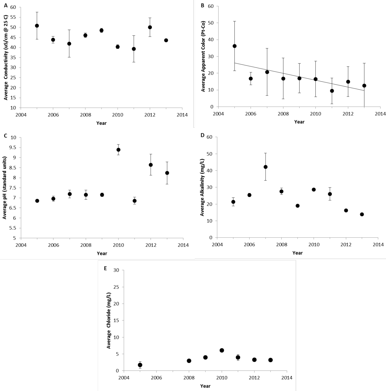
Figure 4. The annual average values of water quality indicators of Fern Lake, 2005-2013. (A) Specific lab conductivity @ 25°C, (B) apparent color, (C) pH, (D) total alkalinity, and (E) chloride concentration. Vertical bars represent one standard deviation of the mean. Significant trends ( P < 0.05 ) are noted with a trend line.
