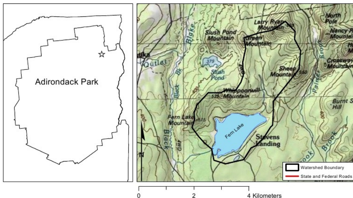
Figure 2. Location and watershed for Fern Lake.
