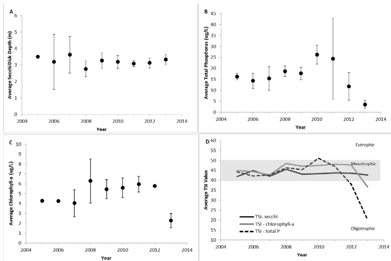
Figure 3. The annual average values of epilimnetic trophic indicators of Fern Lake, 2005-2013. (A) Secchi disk transparency, (B) total phosphorus concentration, (C) chlorophyll-a concentration, and (D) Carlson's Trophic State Index. Vertical bars represent one standard deviation of the mean. Significant trends ( P < 0.05 ) are noted with a trend line.
