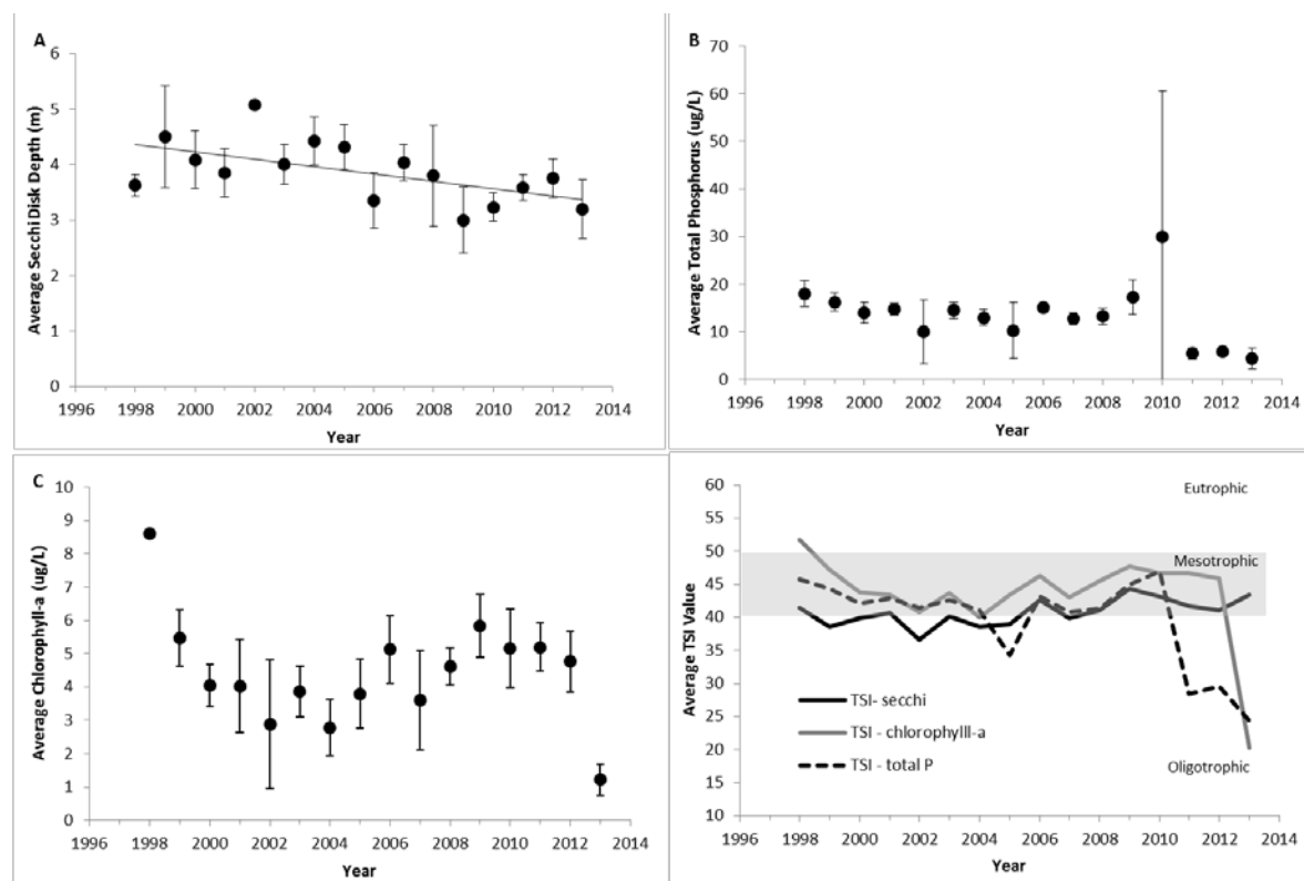
Figure 3. The annual average values of epilimnetic trophic indicators of Cranberry Lake, 1998-2013. (A) Secchi disk transparency, (B) total phosphorus concentration, (C) chlorophyll-a concentration, and (D) Carlson's Trophic State Index. Vertical bars represent one standard deviation of the mean. Significant trends ( P < 0.05 ) are noted with a trend line.
