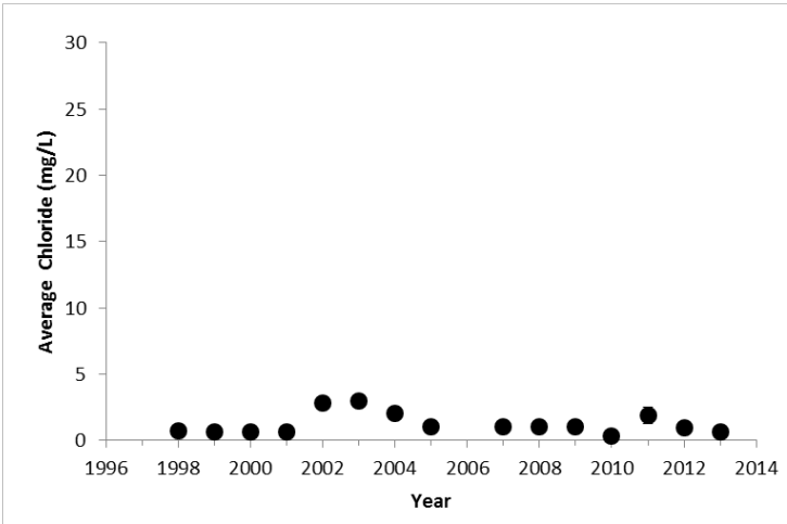
Figure 4. The annual average values of water quality indicators of Cranberry Lake, 1998-2013. (A) Specific lab conductivity @ 25°C, (B) apparent color, (C) pH, (D) total alkalinity, and (E) chloride concentration. Vertical bars represent one standard deviation of the mean. Significant trends ( P < 0.05 ) are noted with a trend line.
