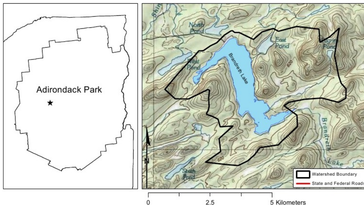
Figure 2. Location and watershed for Brandreth Lake.
