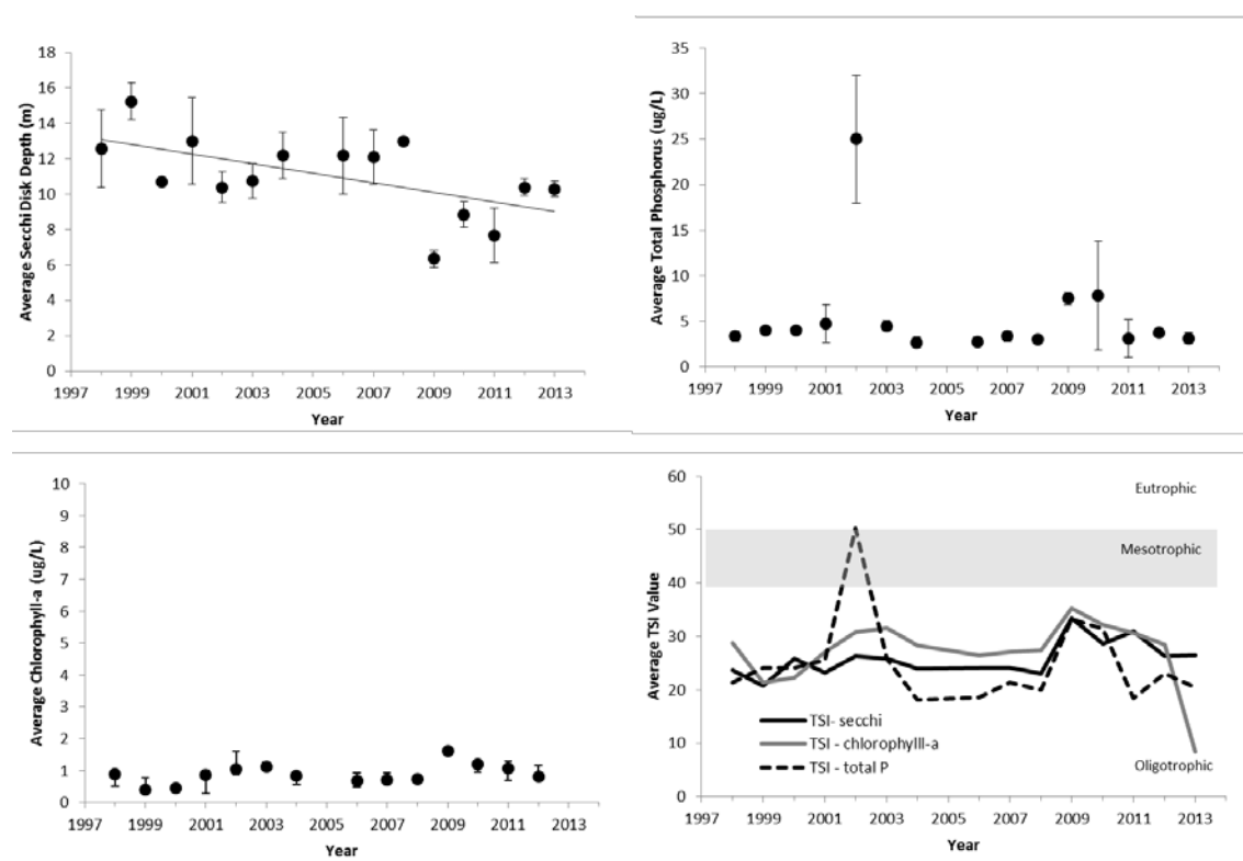
Figure 3. The annual average values of epilimnetic trophic indicators of Brandreth Lake, 1998-2013. (A) Secchi disk transparency, (B) total phosphorus concentration, (C) chlorophyll-a concentration, and (D) Carlson's Trophic State Index. Significant trends ( P < 0.05 ) are indicated with a trend line. Vertical bars represent one standard deviation of the mean.
