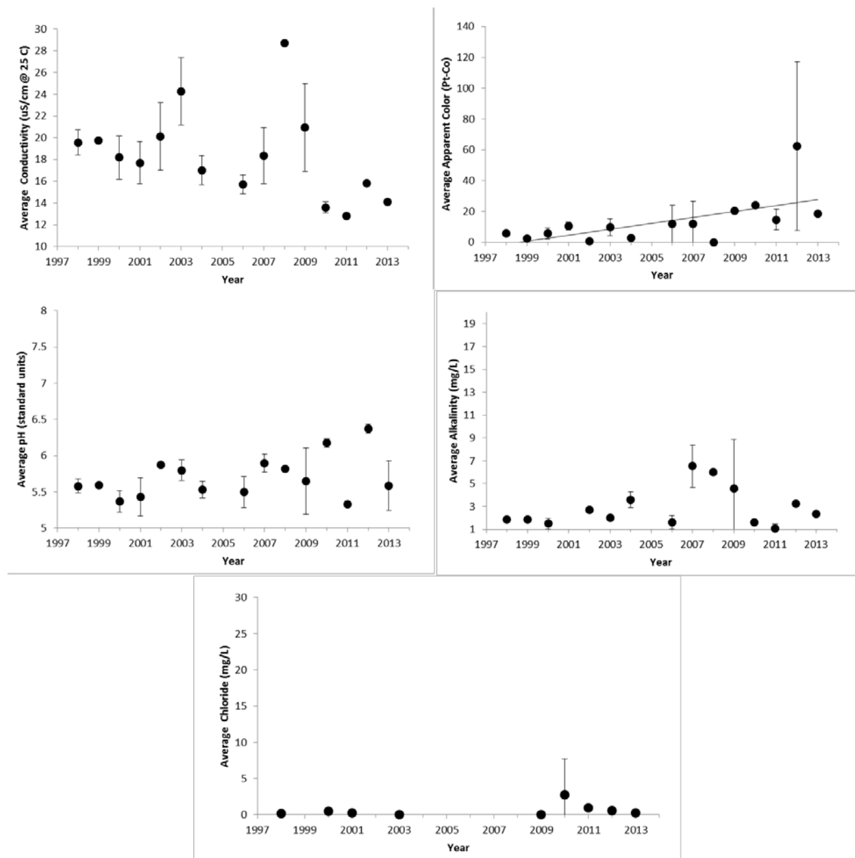
Figure 4. The annual average values of water quality indicators of Brandreth Lake, 1998-2013. (A) Specific lab conductivity @ 25°C, (B) apparent color, (C) pH, (D) total alkalinity, and (E) chloride concentration. Vertical bars represent one standard deviation of the mean. Significant trends ( P < 0.05 ) are noted with a trend line.
